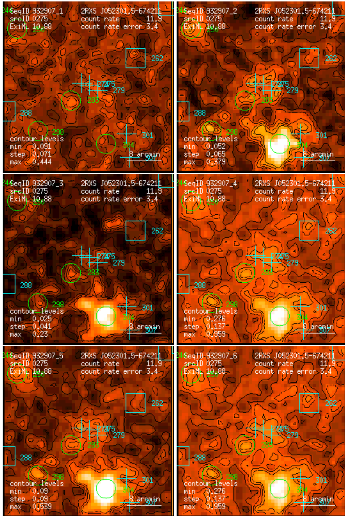
Figure 275: RASS 932907: detection 0275: band rate images, Gaussian filter: (1) PSPC channels 11 – 41, (2) 52 – 90, (3) 91 – 201, (4) 11 – 235, (5) 52 – 201, (6) 11 – 201. Broad band rates in counts/ks. Band rate contour levels in counts/ks/arcmin 2 .
