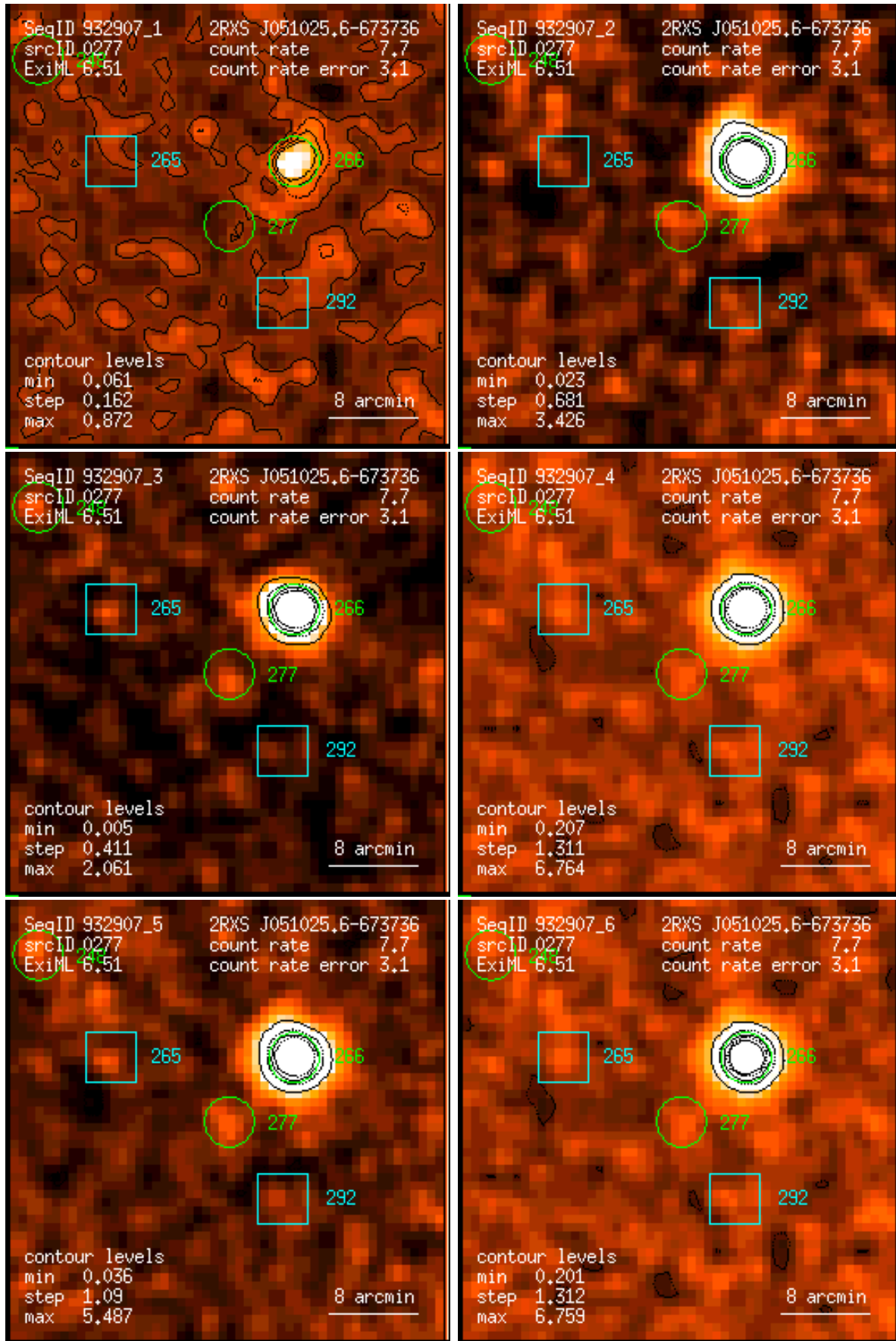
Figure 277: RASS 932907: detection 0277: band rate images, Gaussian filter: (1) PSPC channels 11 – 41, (2) 52 – 90, (3) 91 – 201, (4) 11 – 235, (5) 52 – 201, (6) 11 – 201. Broad band rates in counts/ks. Band rate contour levels in counts/ks/arcmin 2 .
