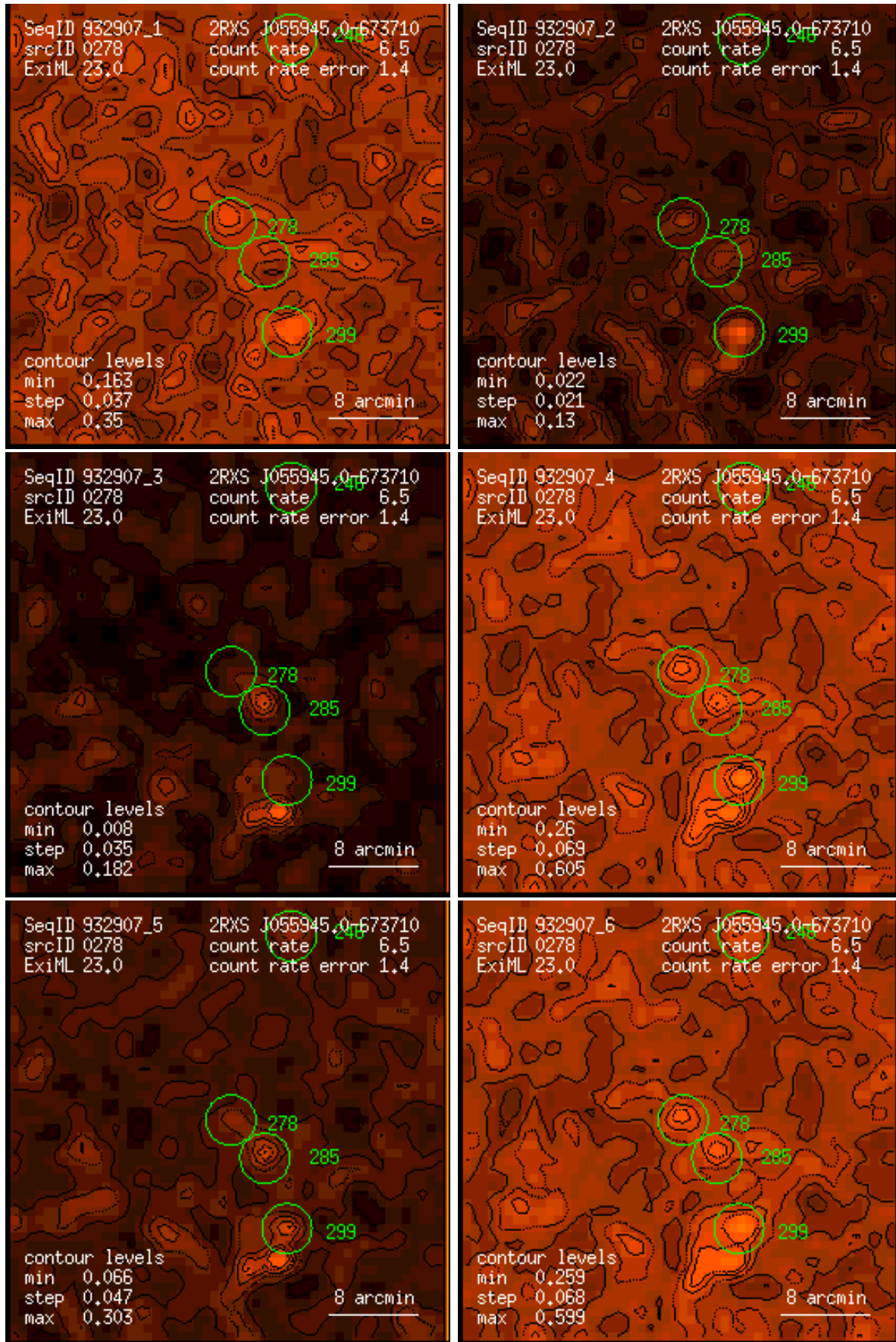
Figure 278: RASS 932907: detection 0278: band rate images, Gaussian filter: (1) PSPC channels 11 – 41, (2) 52 – 90, (3) 91 – 201, (4) 11 – 235, (5) 52 – 201, (6) 11 – 201. Broad band rates in counts/ks. Band rate contour levels in counts/ks/arcmin 2 .
