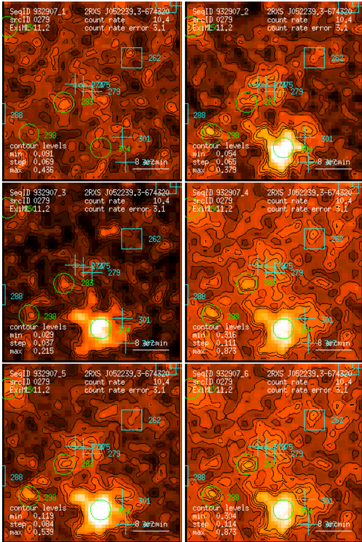
Figure 279: RASS 932907: detection 0279: band rate images, Gaussian filter: (1) PSPC channels 11 – 41, (2) 52 – 90, (3) 91 – 201, (4) 11 – 235, (5) 52 – 201, (6) 11 – 201. Broad band rates in counts/ks. Band rate contour levels in counts/ks/arcmin 2 .
