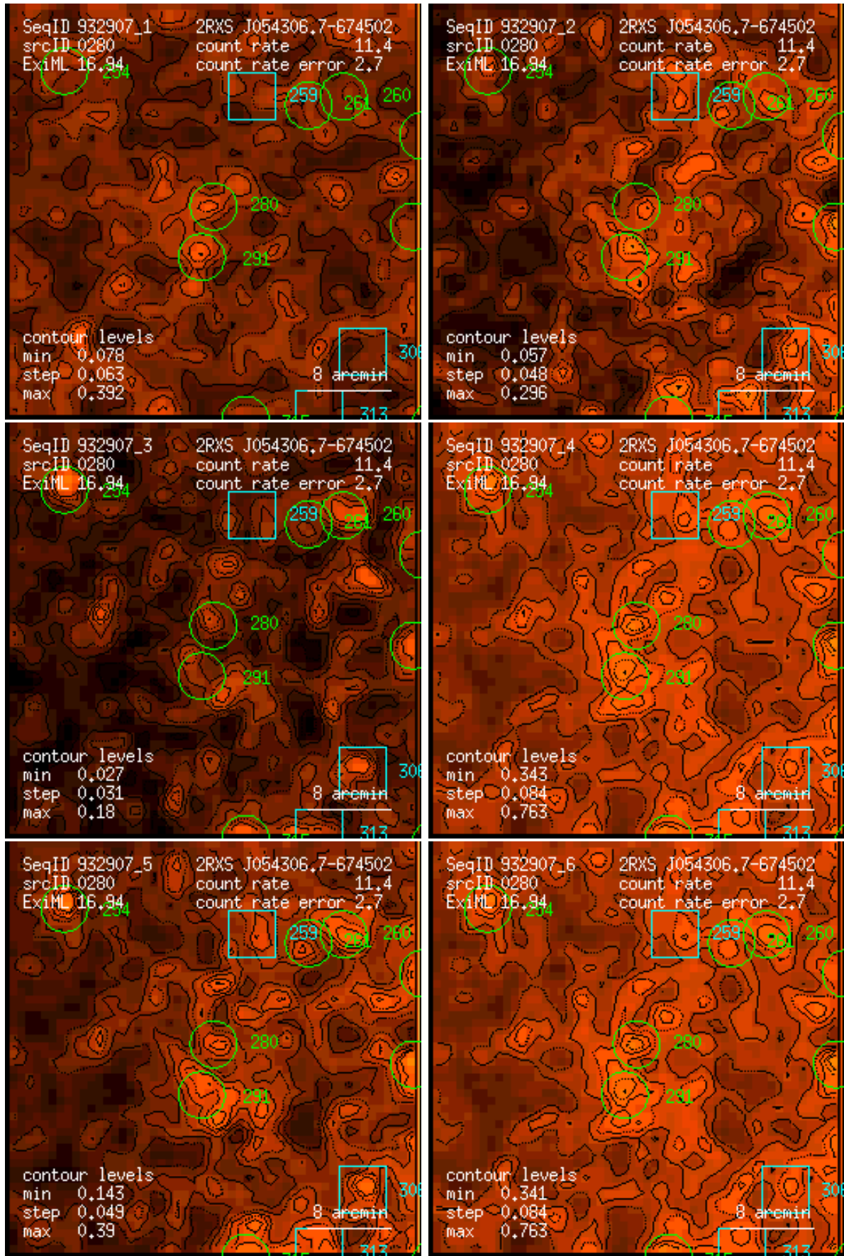
Figure 280: RASS 932907: detection 0280: band rate images, Gaussian filter: (1) PSPC channels 11 – 41, (2) 52 – 90, (3) 91 – 201, (4) 11 – 235, (5) 52 – 201, (6) 11 – 201. Broad band rates in counts/ks. Band rate contour levels in counts/ks/arcmin 2 .
