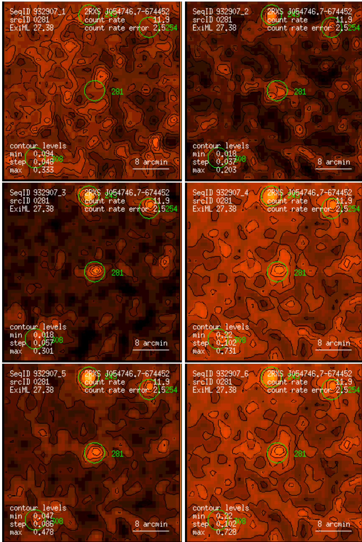
Figure 281: RASS 932907: detection 0281: band rate images, Gaussian filter: (1) PSPC channels 11 – 41, (2) 52 – 90, (3) 91 – 201, (4) 11 – 235, (5) 52 – 201, (6) 11 – 201. Broad band rates in counts/ks. Band rate contour levels in counts/ks/arcmin 2 .
