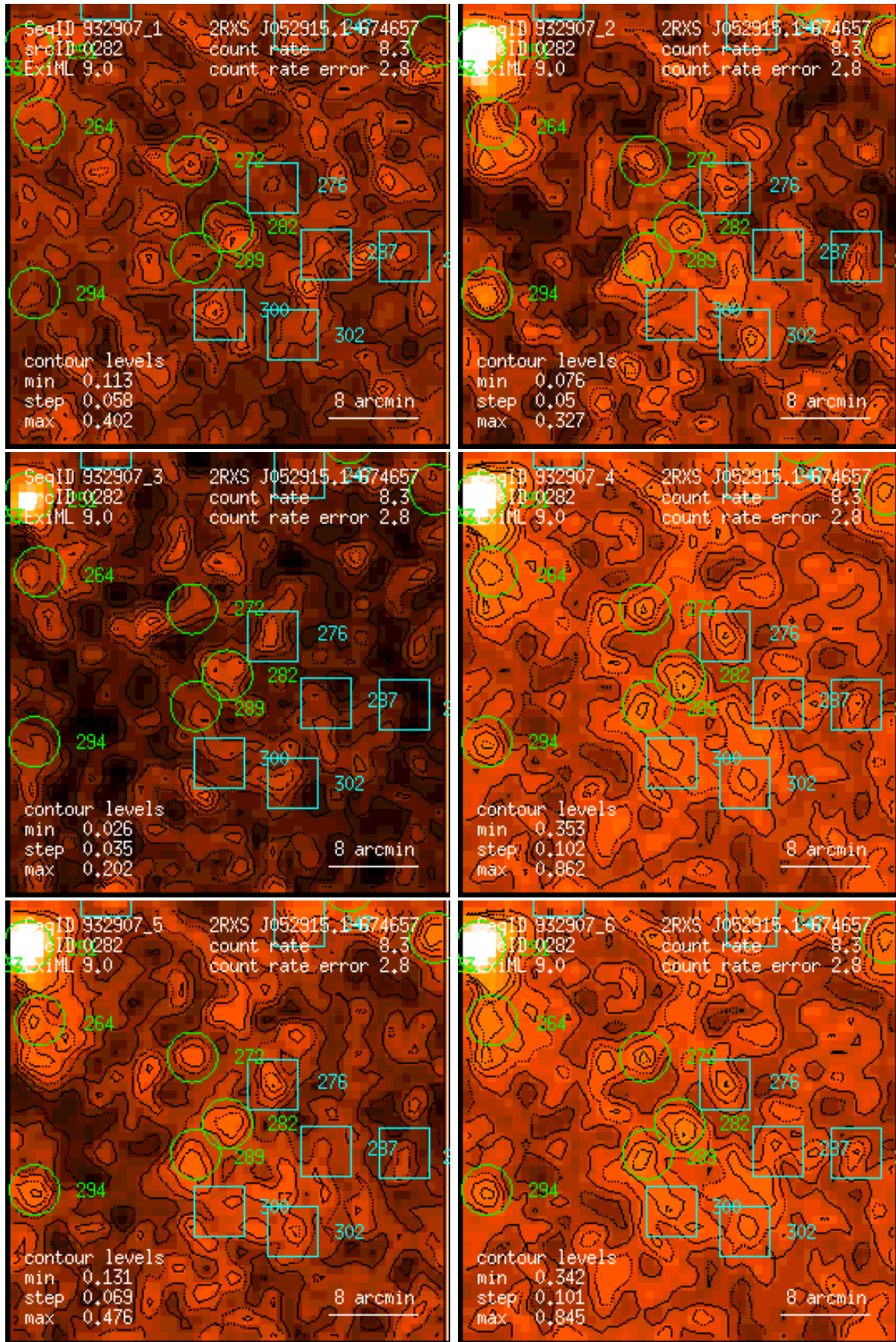
Figure 282: RASS 932907: detection 0282: band rate images, Gaussian filter: (1) PSPC channels 11 – 41, (2) 52 – 90, (3) 91 – 201, (4) 11 – 235, (5) 52 – 201, (6) 11 – 201. Broad band rates in counts/ks. Band rate contour levels in counts/ks/arcmin 2 .
