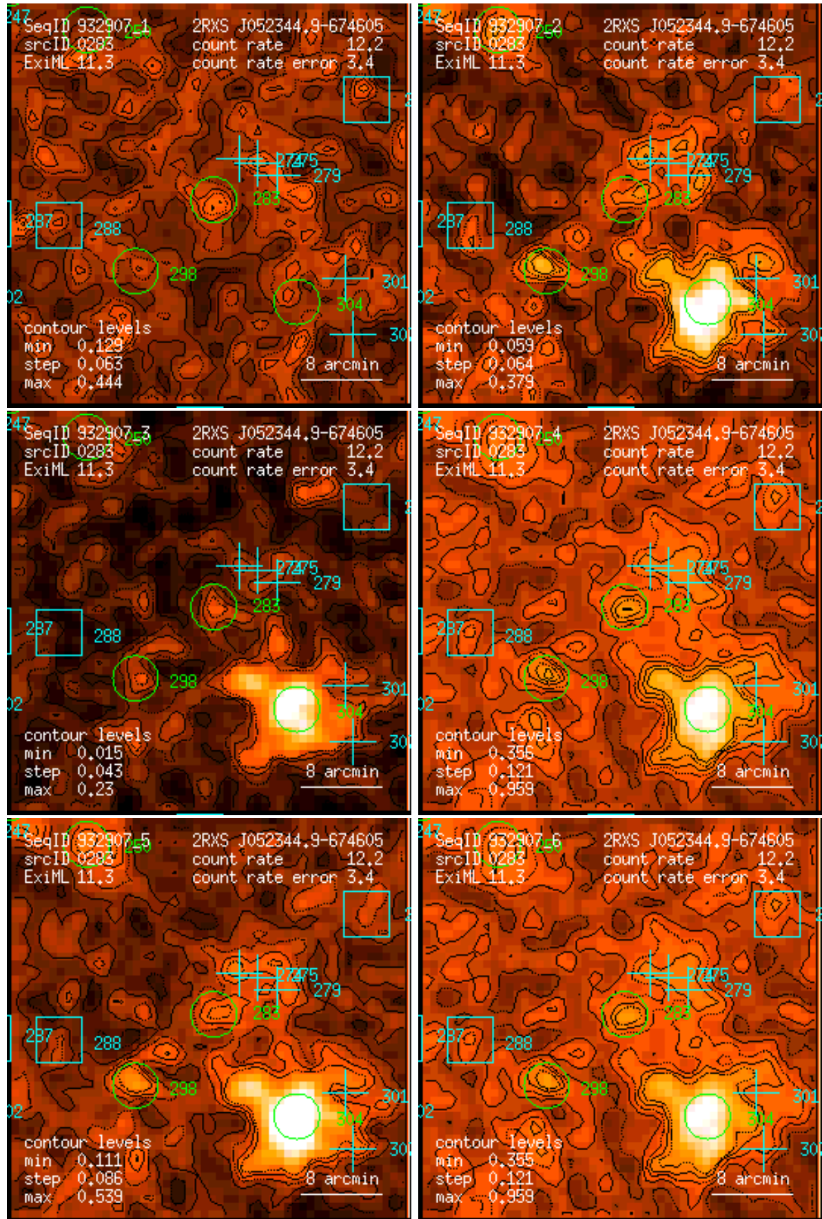
Figure 283: RASS 932907: detection 0283: band rate images, Gaussian filter: (1) PSPC channels 11 – 41, (2) 52 – 90, (3) 91 – 201, (4) 11 – 235, (5) 52 – 201, (6) 11 – 201. Broad band rates in counts/ks. Band rate contour levels in counts/ks/arcmin 2 .
