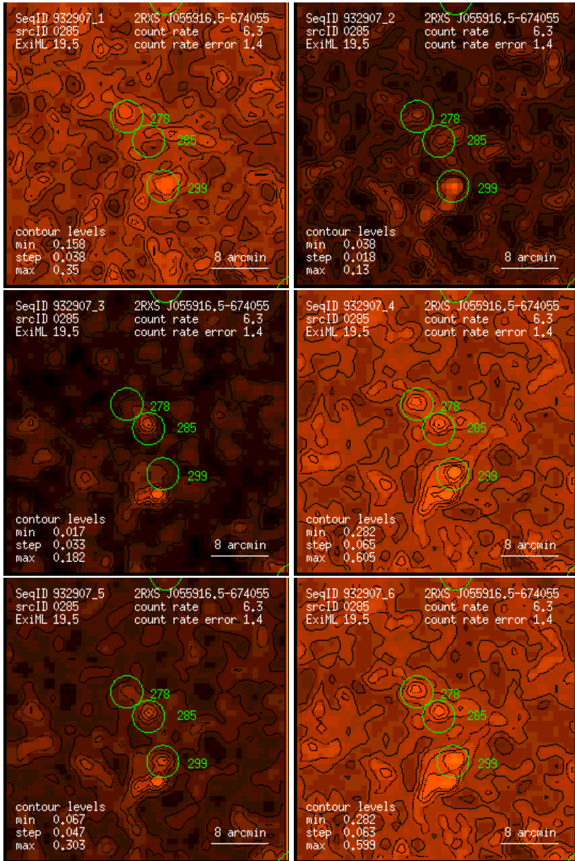
Figure 285: RASS 932907: detection 0285: band rate images, Gaussian filter: (1) PSPC channels 11 – 41, (2) 52 – 90, (3) 91 – 201, (4) 11 – 235, (5) 52 – 201, (6) 11 – 201. Broad band rates in counts/ks. Band rate contour levels in counts/ks/arcmin 2 .
