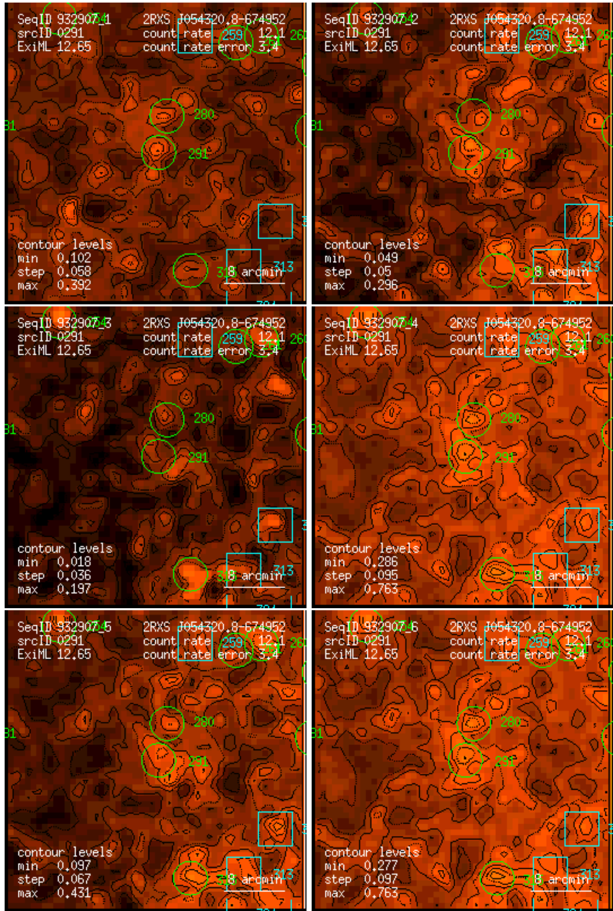
Figure 291: RASS 932907: detection 0291: band rate images, Gaussian filter: (1) PSPC channels 11 – 41, (2) 52 – 90, (3) 91 – 201, (4) 11 – 235, (5) 52 – 201, (6) 11 – 201. Broad band rates in counts/ks. Band rate contour levels in counts/ks/arcmin 2 .
