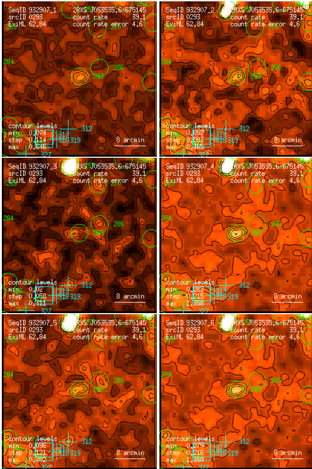
Figure 293: RASS 932907: detection 0293: band rate images, Gaussian filter: (1) PSPC channels 11 – 41, (2) 52 – 90, (3) 91 – 201, (4) 11 – 235, (5) 52 – 201, (6) 11 – 201. Broad band rates in counts/ks. Band rate contour levels in counts/ks/arcmin 2 .
