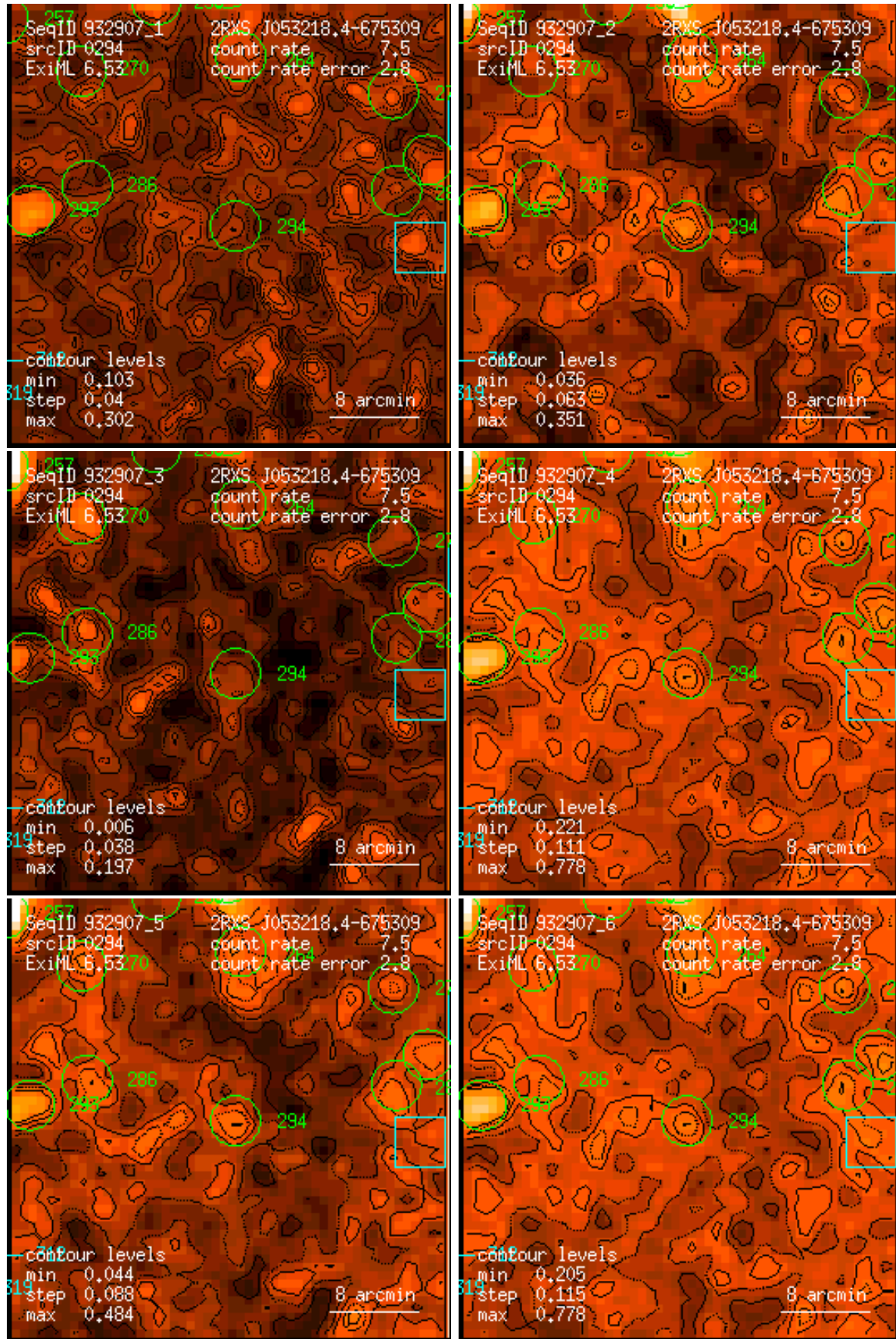
Figure 294: RASS 932907: detection 0294: band rate images, Gaussian filter: (1) PSPC channels 11 – 41, (2) 52 – 90, (3) 91 – 201, (4) 11 – 235, (5) 52 – 201, (6) 11 – 201. Broad band rates in counts/ks. Band rate contour levels in counts/ks/arcmin 2 .
