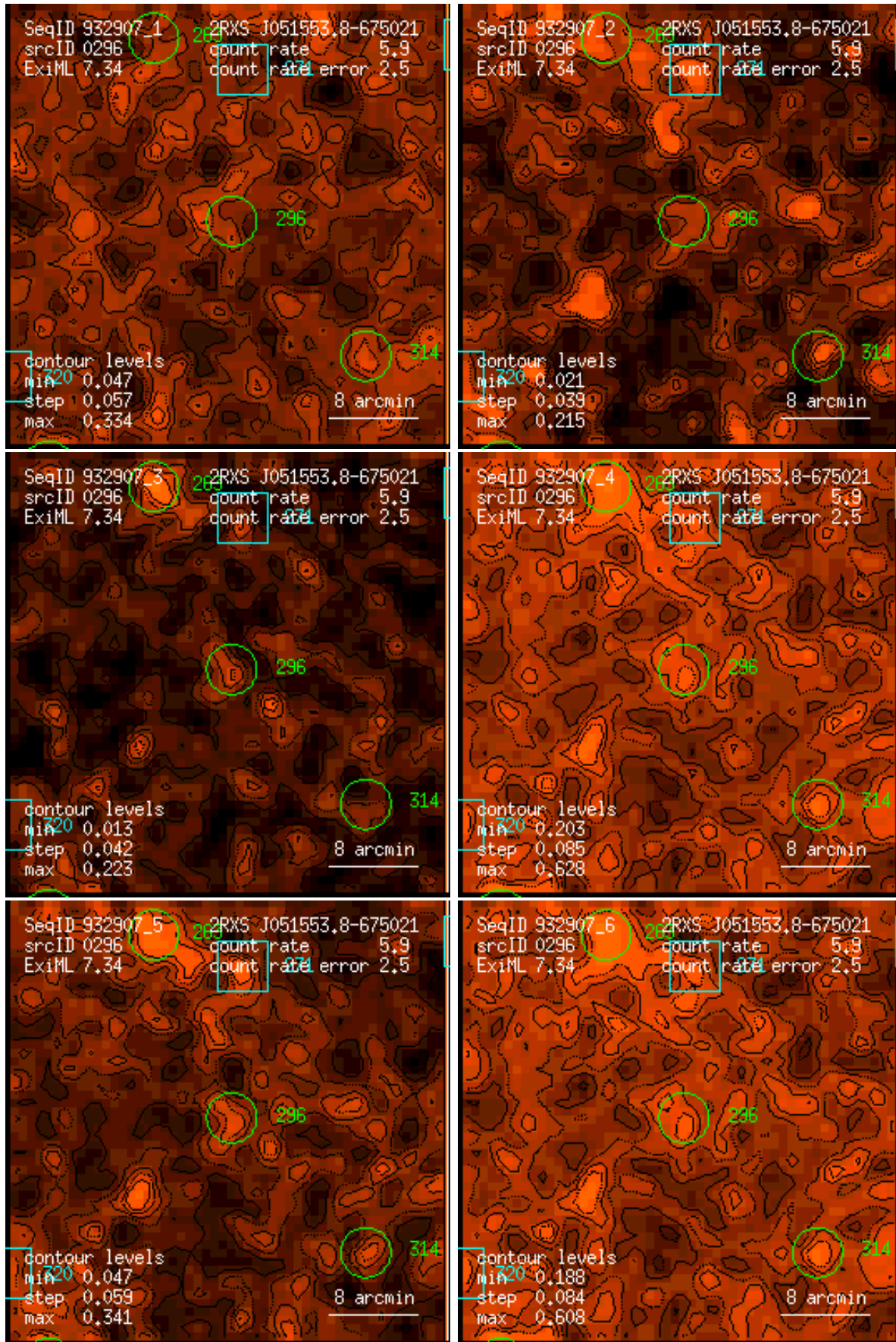
Figure 296: RASS 932907: detection 0296: band rate images, Gaussian filter: (1) PSPC channels 11 – 41, (2) 52 – 90, (3) 91 – 201, (4) 11 – 235, (5) 52 – 201, (6) 11 – 201. Broad band rates in counts/ks. Band rate contour levels in counts/ks/arcmin 2 .
