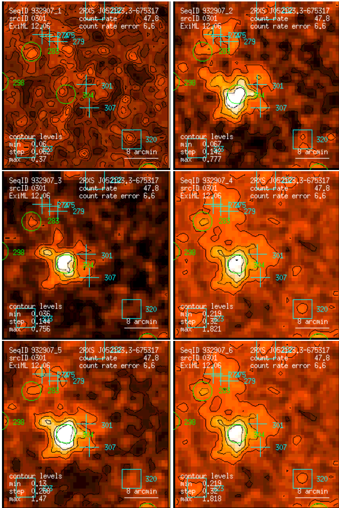
Figure 301: RASS 932907: detection 0301: band rate images, Gaussian filter: (1) PSPC channels 11 – 41, (2) 52 – 90, (3) 91 – 201, (4) 11 – 235, (5) 52 – 201, (6) 11 – 201. Broad band rates in counts/ks. Band rate contour levels in counts/ks/arcmin 2 .
