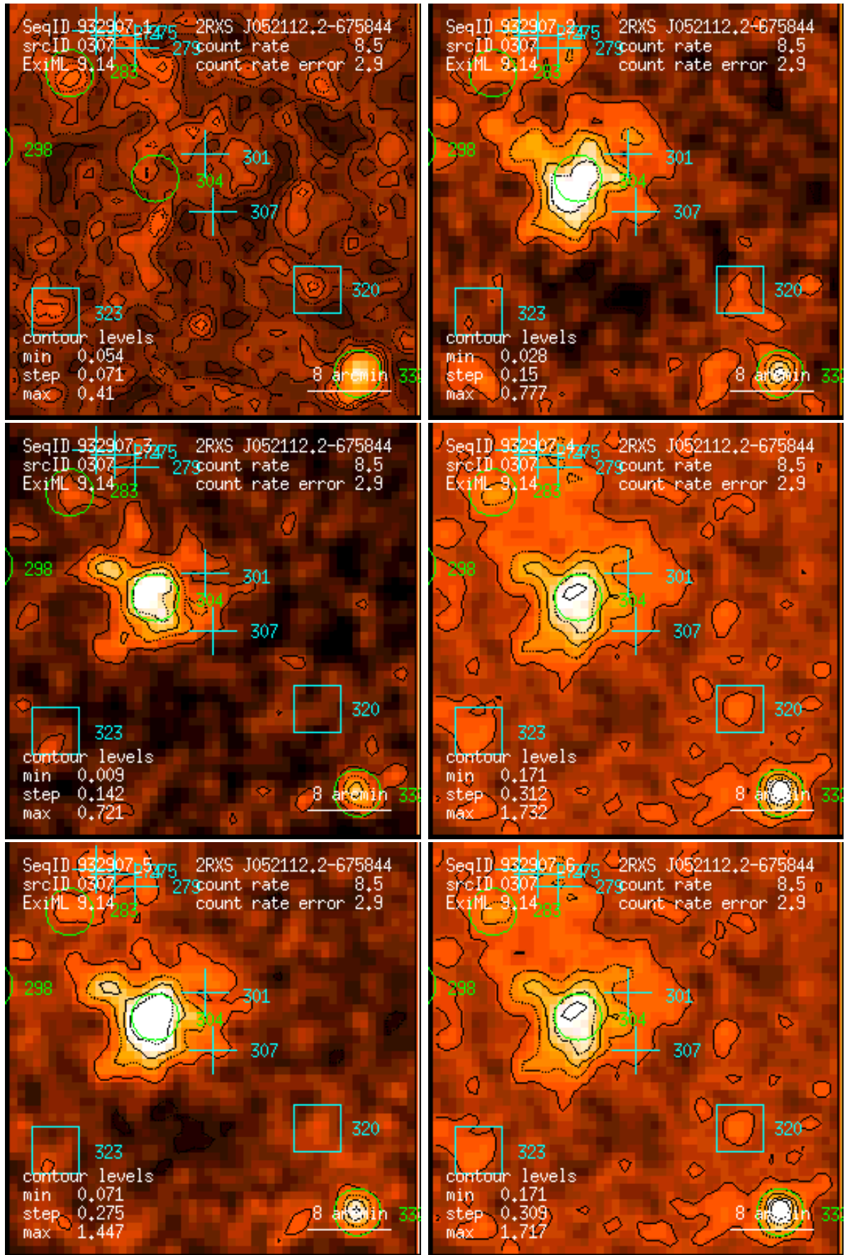
Figure 307: RASS 932907: detection 0307: band rate images, Gaussian filter: (1) PSPC channels 11 – 41, (2) 52 – 90, (3) 91 – 201, (4) 11 – 235, (5) 52 – 201, (6) 11 – 201. Broad band rates in counts/ks. Band rate contour levels in counts/ks/arcmin 2 .
