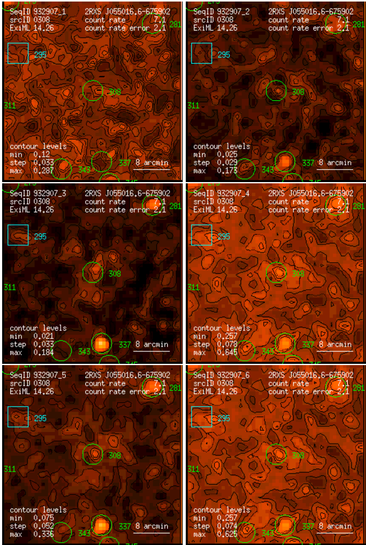
Figure 308: RASS 932907: detection 0308: band rate images, Gaussian filter: (1) PSPC channels 11 – 41, (2) 52 – 90, (3) 91 – 201, (4) 11 – 235, (5) 52 – 201, (6) 11 – 201. Broad band rates in counts/ks. Band rate contour levels in counts/ks/arcmin 2 .
