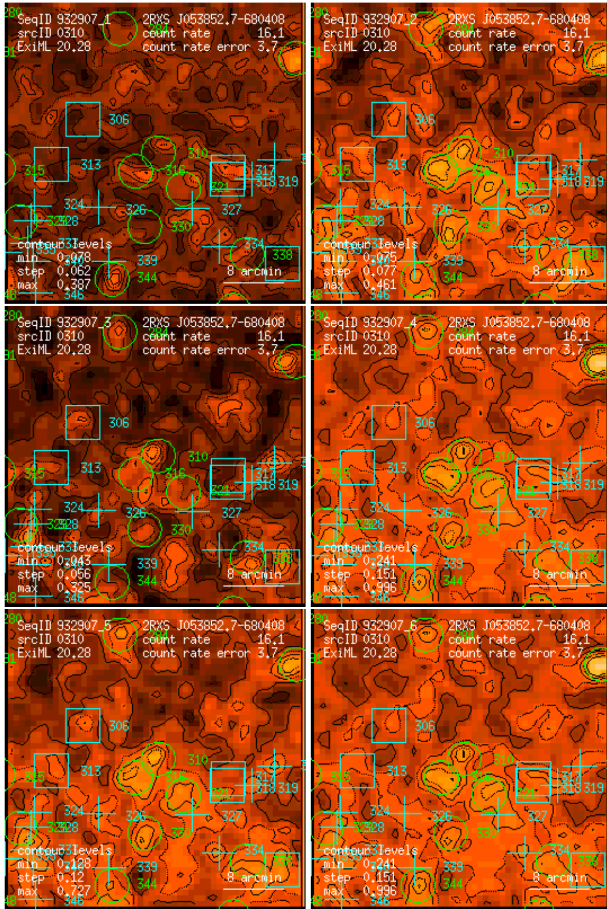
Figure 310: RASS 932907: detection 0310: band rate images, Gaussian filter: (1) PSPC channels 11 – 41, (2) 52 – 90, (3) 91 – 201, (4) 11 – 235, (5) 52 – 201, (6) 11 – 201. Broad band rates in counts/ks. Band rate contour levels in counts/ks/arcmin 2 .
