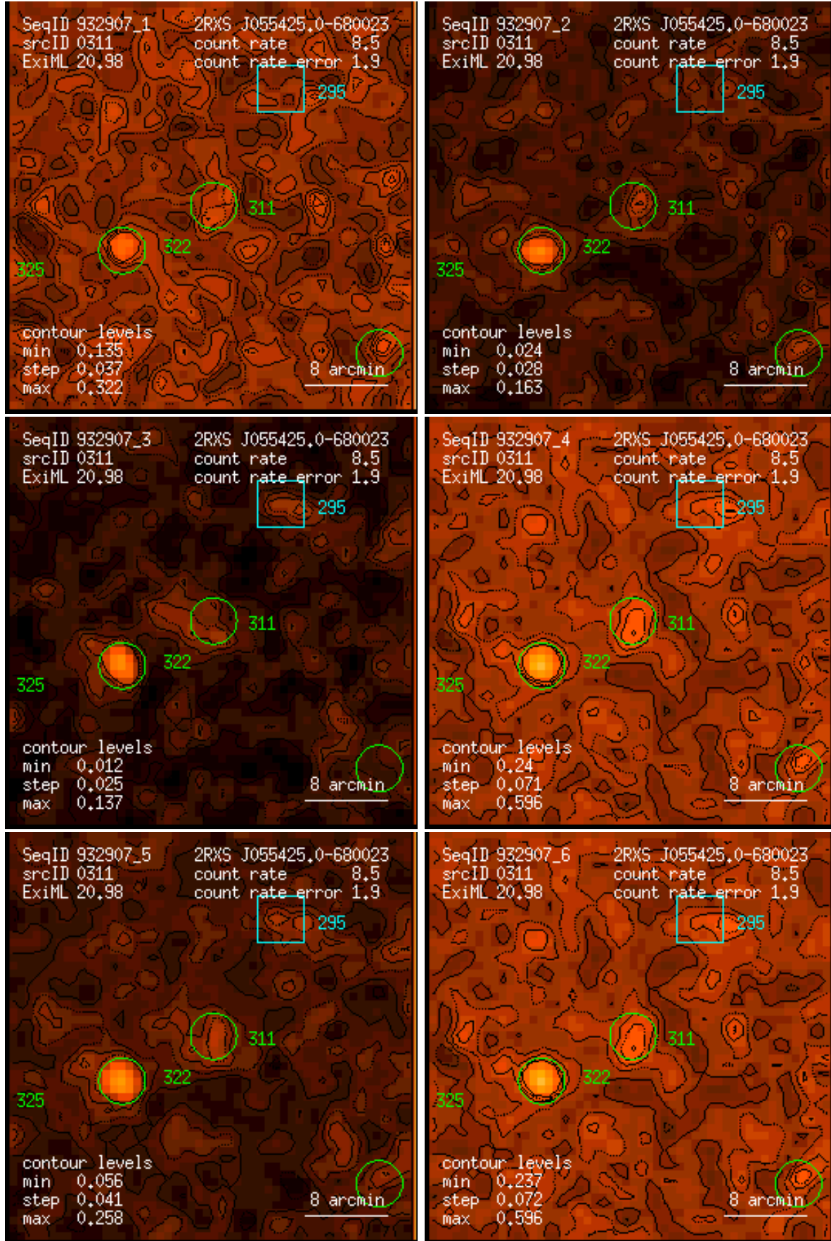
Figure 311: RASS 932907: detection 0311: band rate images, Gaussian filter: (1) PSPC channels 11 – 41, (2) 52 – 90, (3) 91 – 201, (4) 11 – 235, (5) 52 – 201, (6) 11 – 201. Broad band rates in counts/ks. Band rate contour levels in counts/ks/arcmin 2 .
