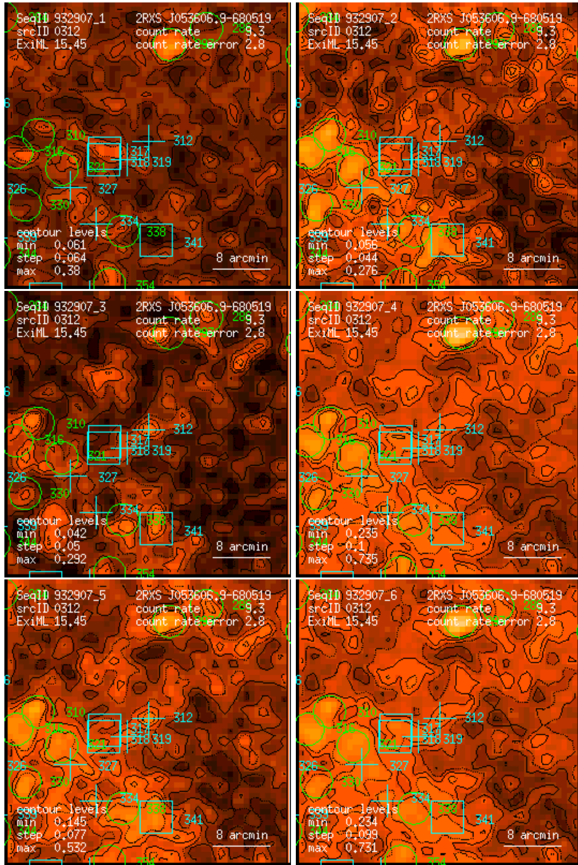
Figure 312: RASS 932907: detection 0312: band rate images, Gaussian filter: (1) PSPC channels 11 – 41, (2) 52 – 90, (3) 91 – 201, (4) 11 – 235, (5) 52 – 201, (6) 11 – 201. Broad band rates in counts/ks. Band rate contour levels in counts/ks/arcmin 2 .
