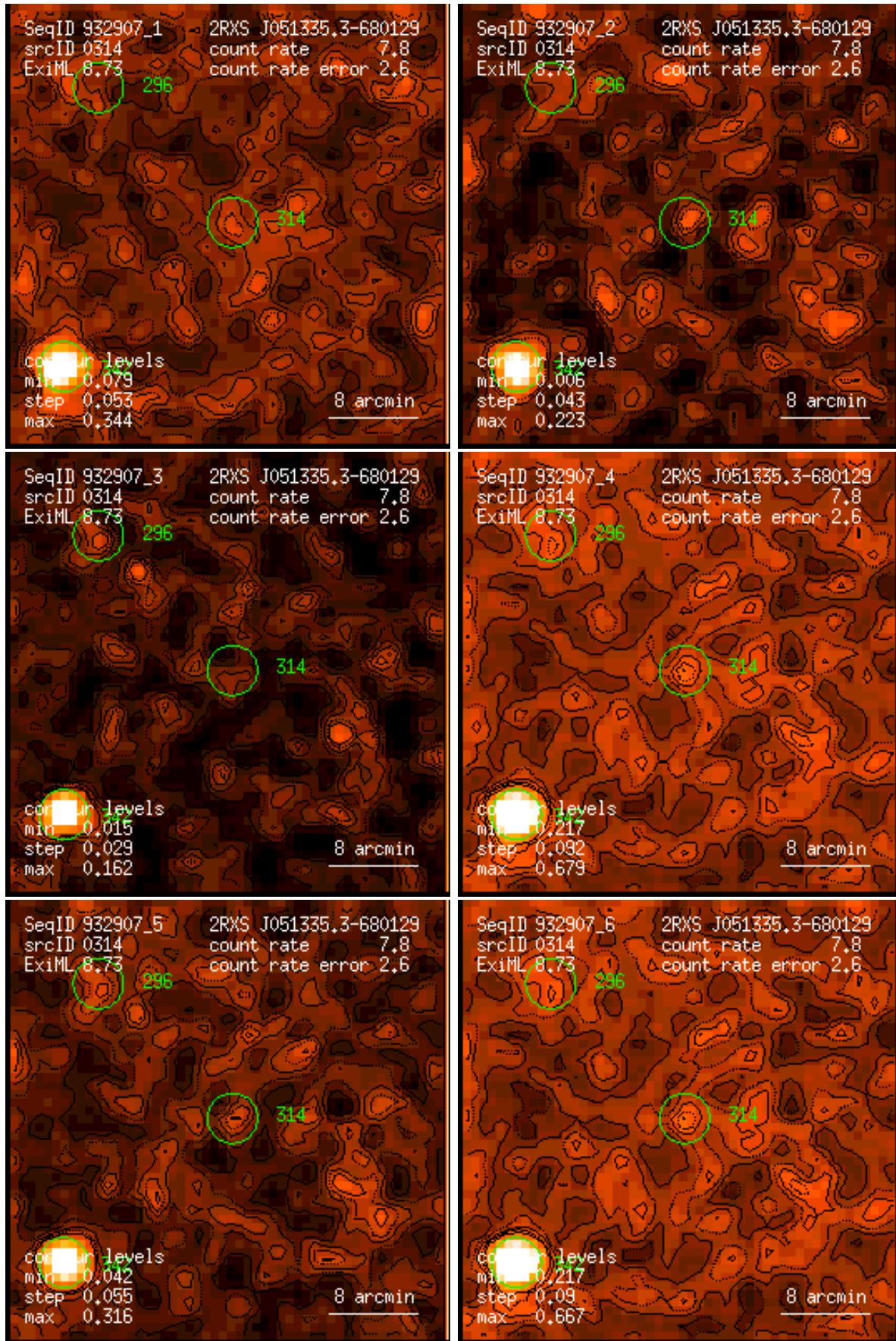
Figure 314: RASS 932907: detection 0314: band rate images, Gaussian filter: (1) PSPC channels 11 – 41, (2) 52 – 90, (3) 91 – 201, (4) 11 – 235, (5) 52 – 201, (6) 11 – 201. Broad band rates in counts/ks. Band rate contour levels in counts/ks/arcmin 2 .
