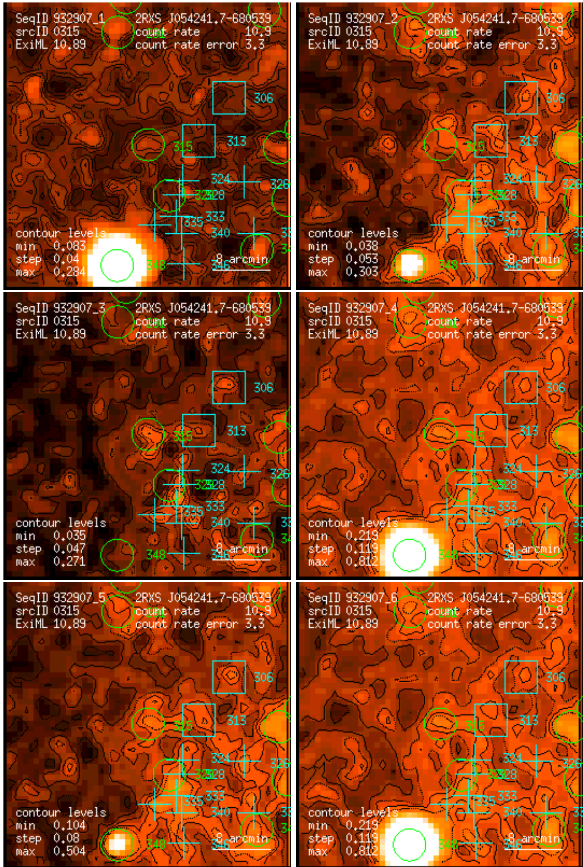
Figure 315: RASS 932907: detection 0315: band rate images, Gaussian filter: (1) PSPC channels 11 – 41, (2) 52 – 90, (3) 91 – 201, (4) 11 – 235, (5) 52 – 201, (6) 11 – 201. Broad band rates in counts/ks. Band rate contour levels in counts/ks/arcmin 2 .
