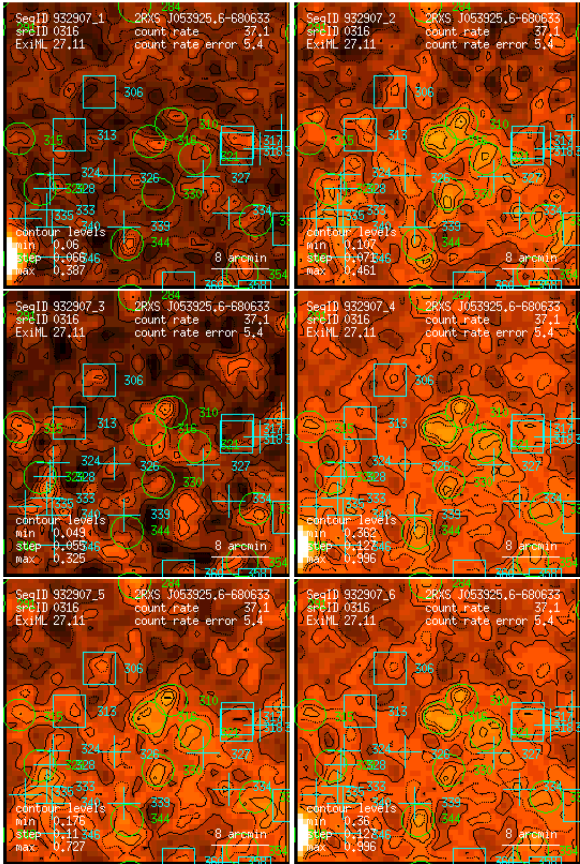
Figure 316: RASS 932907: detection 0316: band rate images, Gaussian filter: (1) PSPC channels 11 – 41, (2) 52 – 90, (3) 91 – 201, (4) 11 – 235, (5) 52 – 201, (6) 11 – 201. Broad band rates in counts/ks. Band rate contour levels in counts/ks/arcmin 2 .
