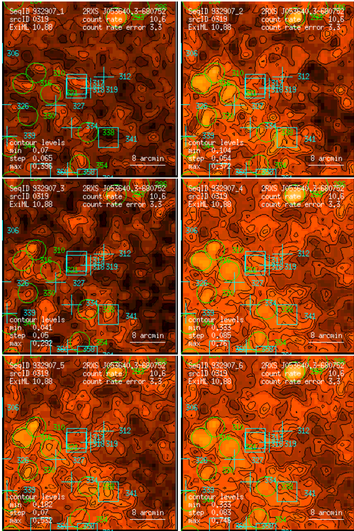
Figure 319: RASS 932907: detection 0319: band rate images, Gaussian filter: (1) PSPC channels 11 – 41, (2) 52 – 90, (3) 91 – 201, (4) 11 – 235, (5) 52 – 201, (6) 11 – 201. Broad band rates in counts/ks. Band rate contour levels in counts/ks/arcmin 2 .
