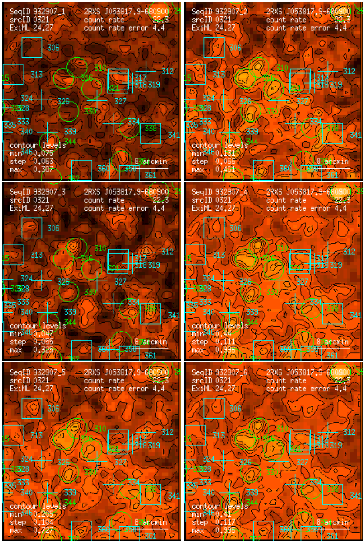
Figure 321: RASS 932907: detection 0321: band rate images, Gaussian filter: (1) PSPC channels 11 – 41, (2) 52 – 90, (3) 91 – 201, (4) 11 – 235, (5) 52 – 201, (6) 11 – 201. Broad band rates in counts/ks. Band rate contour levels in counts/ks/arcmin 2 .
