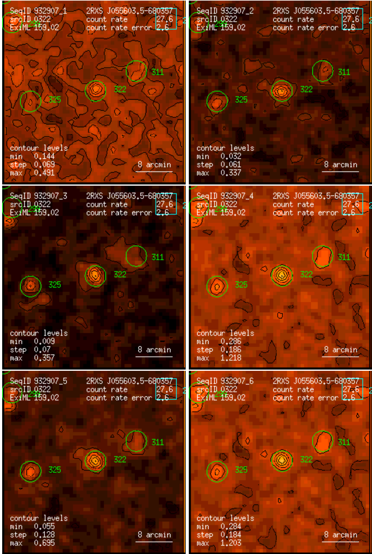
Figure 322: RASS 932907: detection 0322: band rate images, Gaussian filter: (1) PSPC channels 11 – 41, (2) 52 – 90, (3) 91 – 201, (4) 11 – 235, (5) 52 – 201, (6) 11 – 201. Broad band rates in counts/ks. Band rate contour levels in counts/ks/arcmin 2 .
