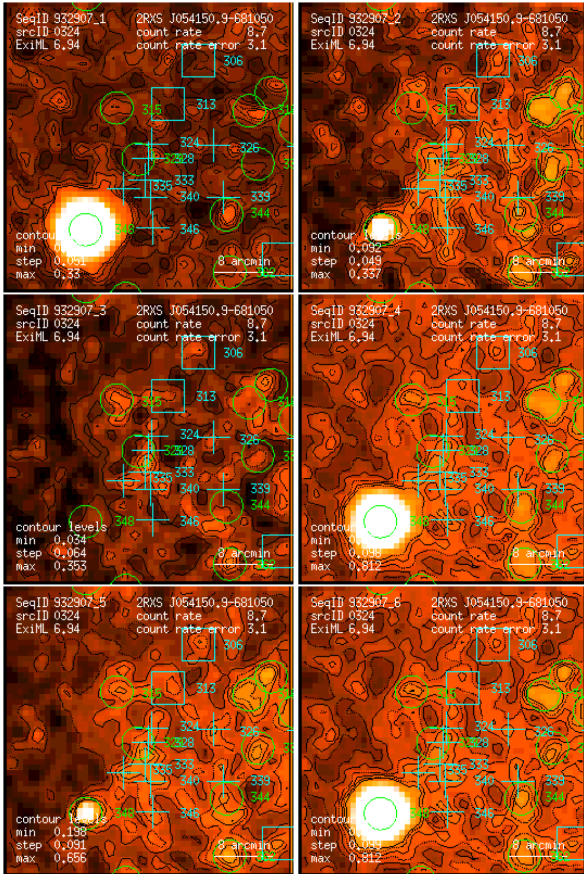
Figure 324: RASS 932907: detection 0324: band rate images, Gaussian filter: (1) PSPC channels 11 – 41, (2) 52 – 90, (3) 91 – 201, (4) 11 – 235, (5) 52 – 201, (6) 11 – 201. Broad band rates in counts/ks. Band rate contour levels in counts/ks/arcmin 2 .
