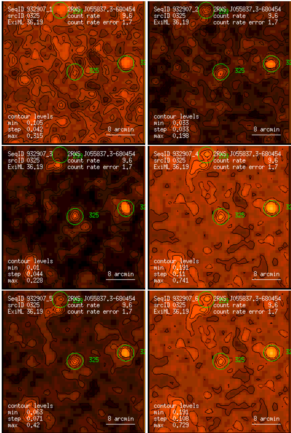
Figure 325: RASS 932907: detection 0325: band rate images, Gaussian filter: (1) PSPC channels 11 – 41, (2) 52 – 90, (3) 91 – 201, (4) 11 – 235, (5) 52 – 201, (6) 11 – 201. Broad band rates in counts/ks. Band rate contour levels in counts/ks/arcmin 2 .
