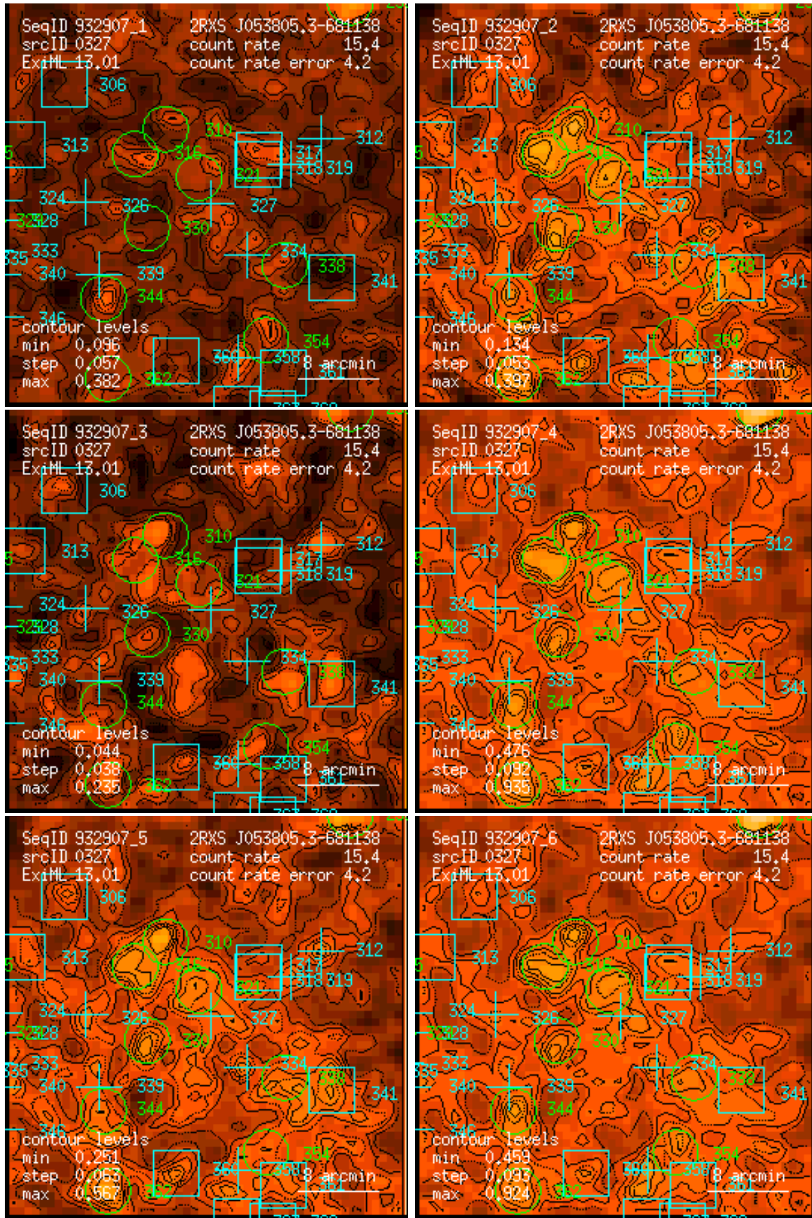
Figure 327: RASS 932907: detection 0327: band rate images, Gaussian filter: (1) PSPC channels 11 – 41, (2) 52 – 90, (3) 91 – 201, (4) 11 – 235, (5) 52 – 201, (6) 11 – 201. Broad band rates in counts/ks. Band rate contour levels in counts/ks/arcmin 2 .
