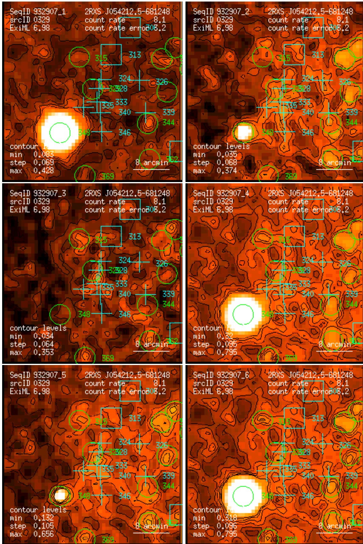
Figure 329: RASS 932907: detection 0329: band rate images, Gaussian filter: (1) PSPC channels 11 – 41, (2) 52 – 90, (3) 91 – 201, (4) 11 – 235, (5) 52 – 201, (6) 11 – 201. Broad band rates in counts/ks. Band rate contour levels in counts/ks/arcmin 2 .
