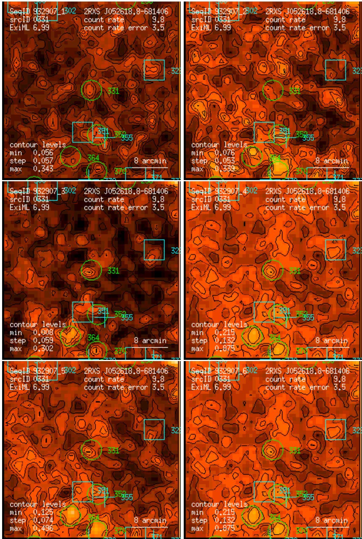
Figure 331: RASS 932907: detection 0331: band rate images, Gaussian filter: (1) PSPC channels 11 – 41, (2) 52 – 90, (3) 91 – 201, (4) 11 – 235, (5) 52 – 201, (6) 11 – 201. Broad band rates in counts/ks. Band rate contour levels in counts/ks/arcmin 2 .
