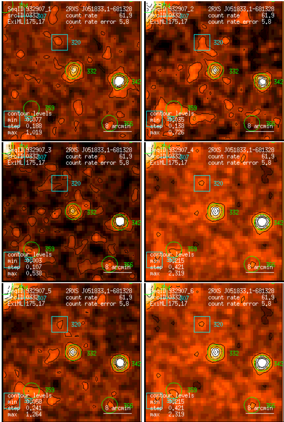
Figure 332: RASS 932907: detection 0332: band rate images, Gaussian filter: (1) PSPC channels 11 – 41, (2) 52 – 90, (3) 91 – 201, (4) 11 – 235, (5) 52 – 201, (6) 11 – 201. Broad band rates in counts/ks. Band rate contour levels in counts/ks/arcmin 2 .
