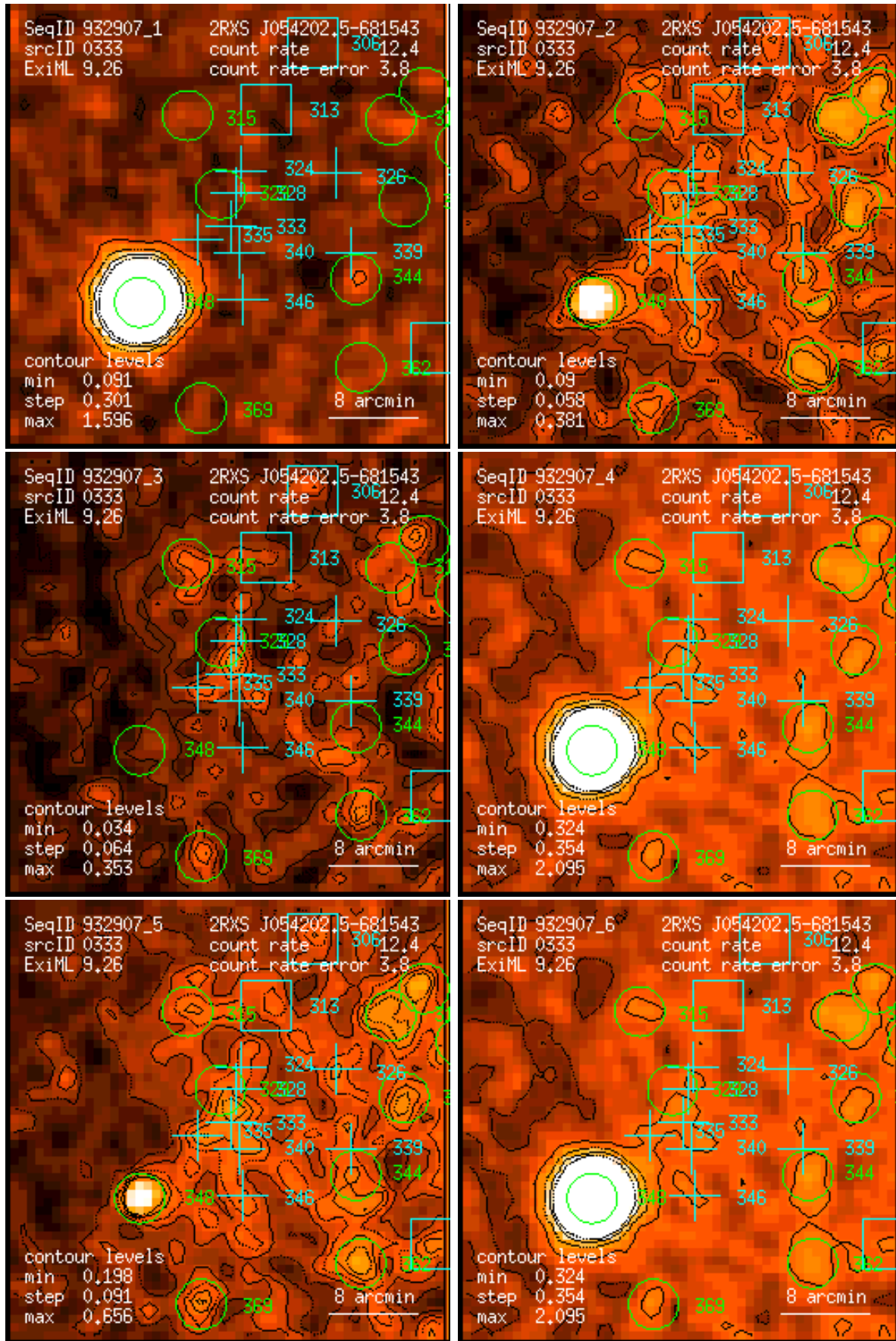
Figure 333: RASS 932907: detection 0333: band rate images, Gaussian filter: (1) PSPC channels 11 – 41, (2) 52 – 90, (3) 91 – 201, (4) 11 – 235, (5) 52 – 201, (6) 11 – 201. Broad band rates in counts/ks. Band rate contour levels in counts/ks/arcmin 2 .
