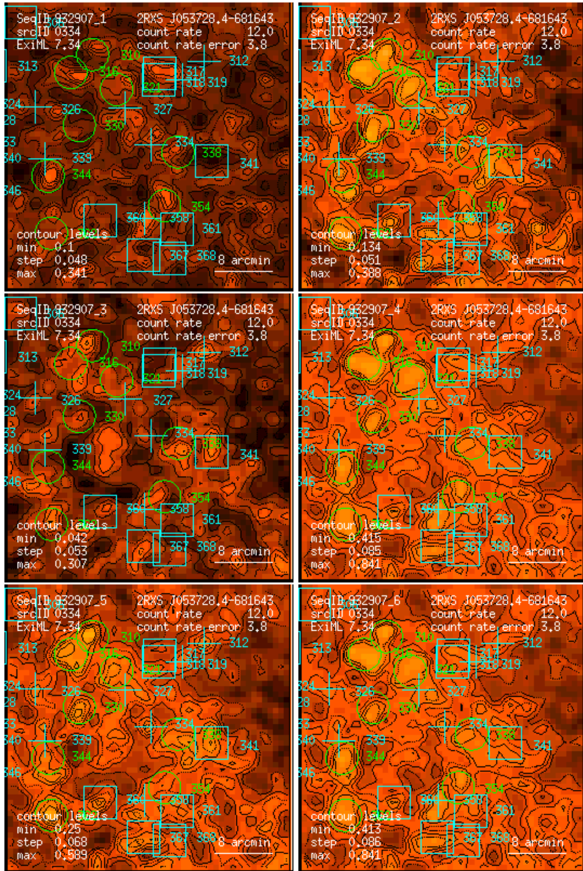
Figure 334: RASS 932907: detection 0334: band rate images, Gaussian filter: (1) PSPC channels 11 – 41, (2) 52 – 90, (3) 91 – 201, (4) 11 – 235, (5) 52 – 201, (6) 11 – 201. Broad band rates in counts/ks. Band rate contour levels in counts/ks/arcmin 2 .
