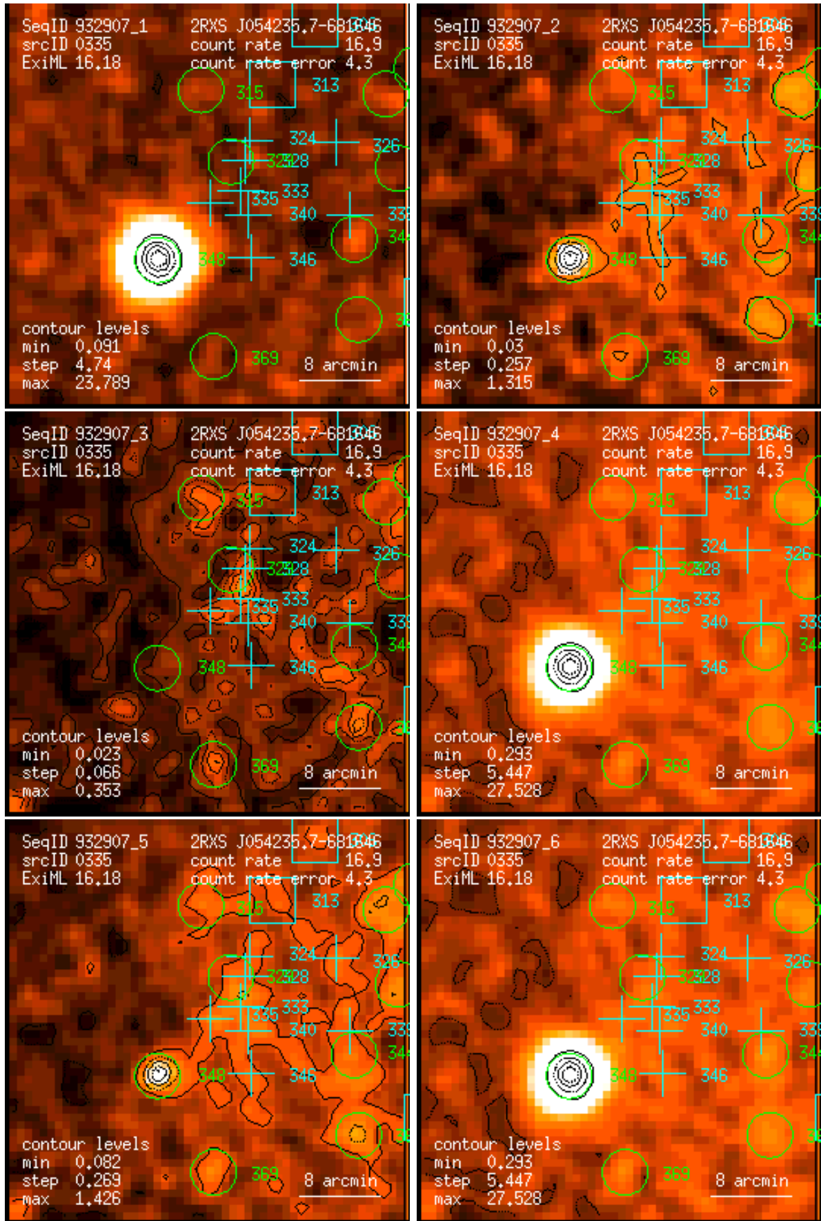
Figure 335: RASS 932907: detection 0335: band rate images, Gaussian filter: (1) PSPC channels 11 – 41, (2) 52 – 90, (3) 91 – 201, (4) 11 – 235, (5) 52 – 201, (6) 11 – 201. Broad band rates in counts/ks. Band rate contour levels in counts/ks/arcmin 2 .
