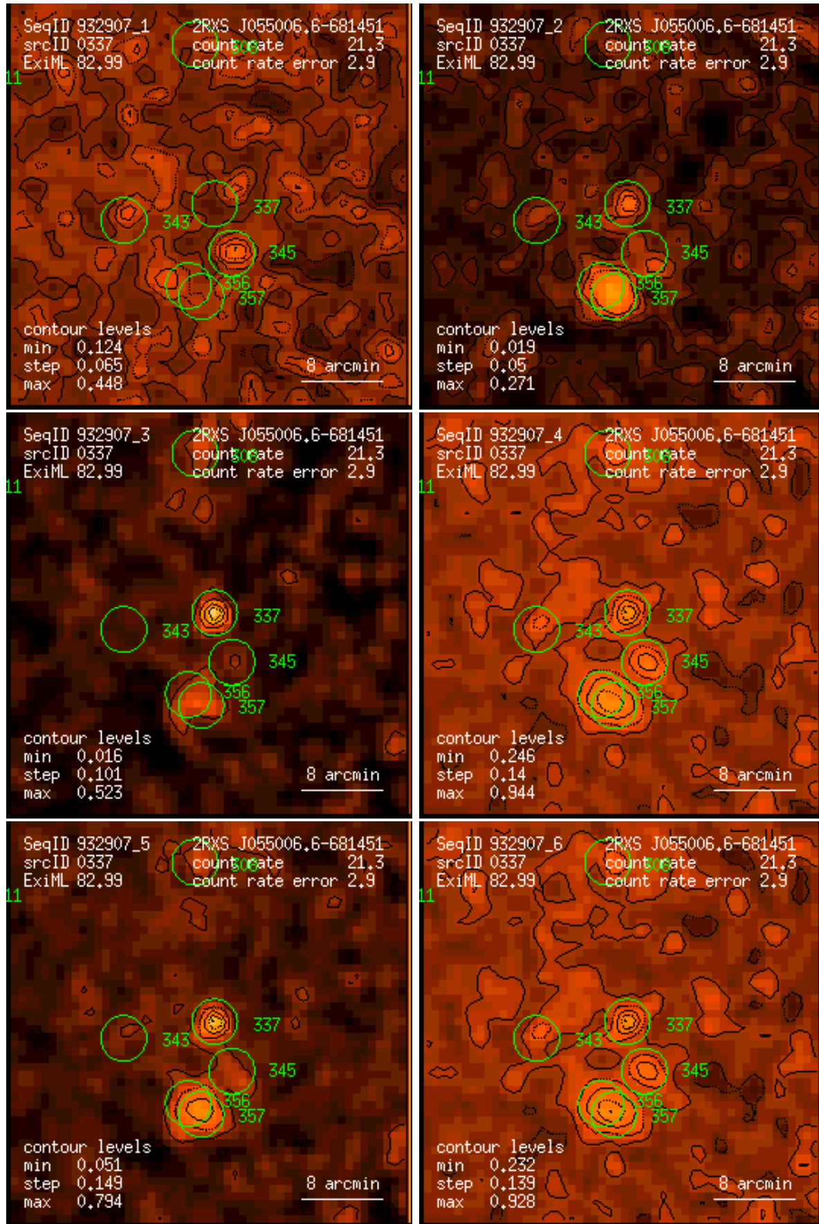
Figure 337: RASS 932907: detection 0337: band rate images, Gaussian filter: (1) PSPC channels 11 – 41, (2) 52 – 90, (3) 91 – 201, (4) 11 – 235, (5) 52 – 201, (6) 11 – 201. Broad band rates in counts/ks. Band rate contour levels in counts/ks/arcmin 2 .
