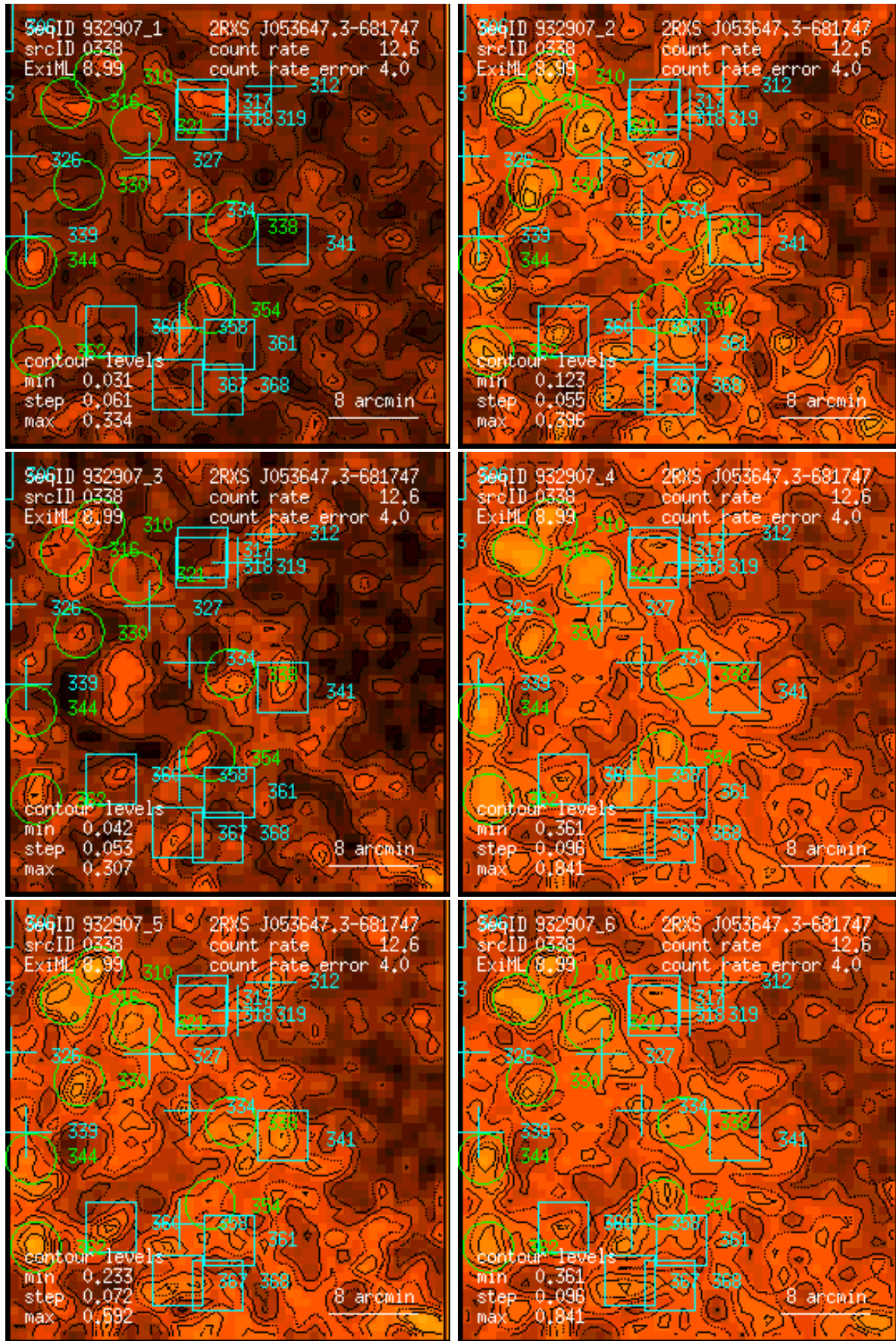
Figure 338: RASS 932907: detection 0338: band rate images, Gaussian filter: (1) PSPC channels 11 – 41, (2) 52 – 90, (3) 91 – 201, (4) 11 – 235, (5) 52 – 201, (6) 11 – 201. Broad band rates in counts/ks. Band rate contour levels in counts/ks/arcmin 2 .
