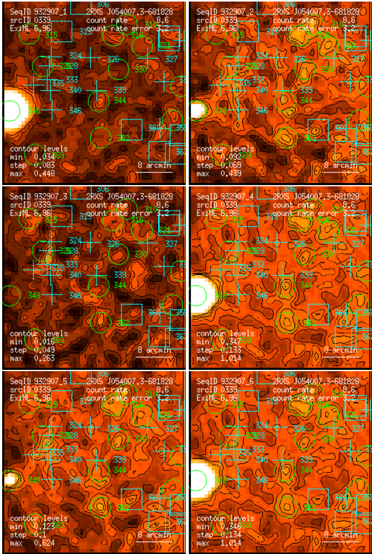
Figure 339: RASS 932907: detection 0339: band rate images, Gaussian filter: (1) PSPC channels 11 – 41, (2) 52 – 90, (3) 91 – 201, (4) 11 – 235, (5) 52 – 201, (6) 11 – 201. Broad band rates in counts/ks. Band rate contour levels in counts/ks/arcmin 2 .
