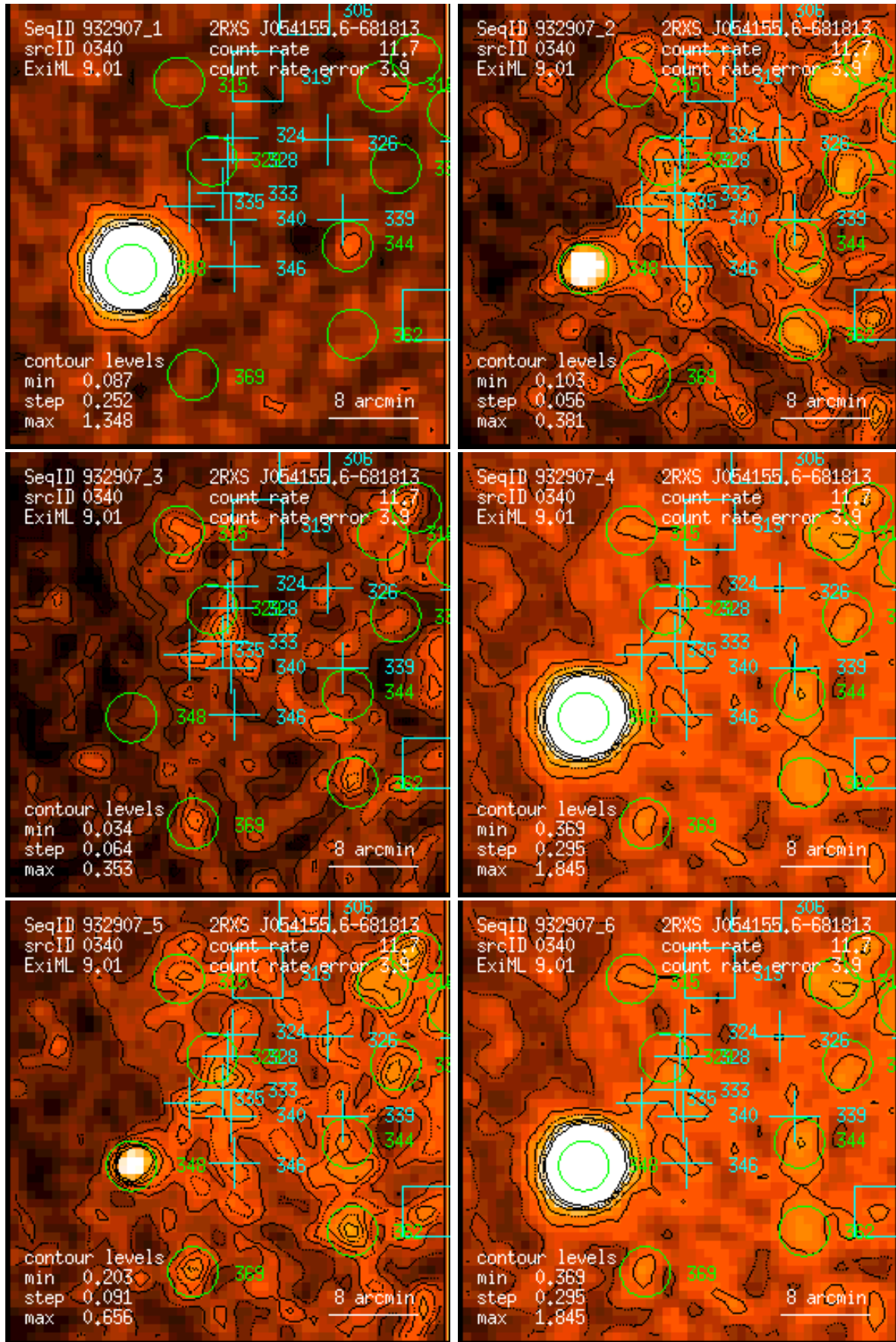
Figure 340: RASS 932907: detection 0340: band rate images, Gaussian filter: (1) PSPC channels 11 – 41, (2) 52 – 90, (3) 91 – 201, (4) 11 – 235, (5) 52 – 201, (6) 11 – 201. Broad band rates in counts/ks. Band rate contour levels in counts/ks/arcmin 2 .
