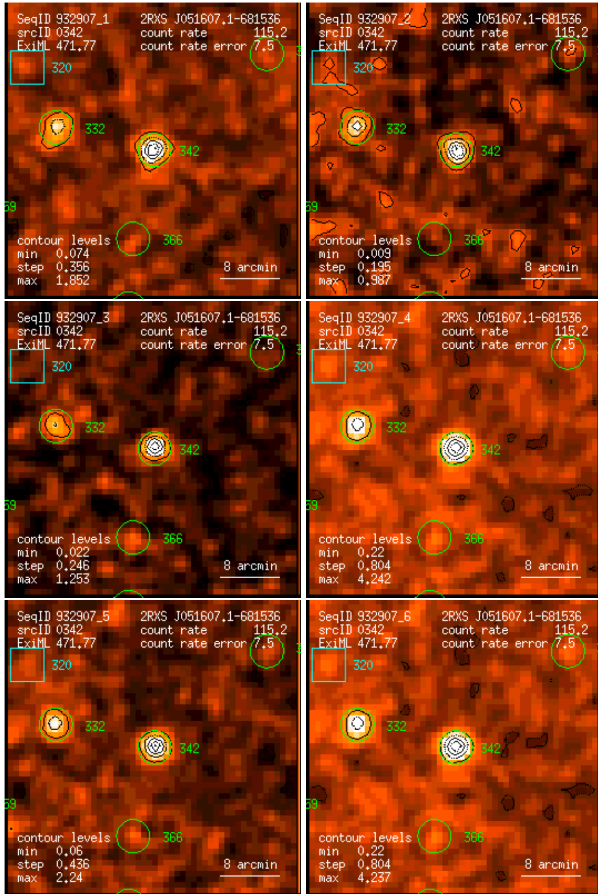
Figure 342: RASS 932907: detection 0342: band rate images, Gaussian filter: (1) PSPC channels 11 – 41, (2) 52 – 90, (3) 91 – 201, (4) 11 – 235, (5) 52 – 201, (6) 11 – 201. Broad band rates in counts/ks. Band rate contour levels in counts/ks/arcmin 2 .
