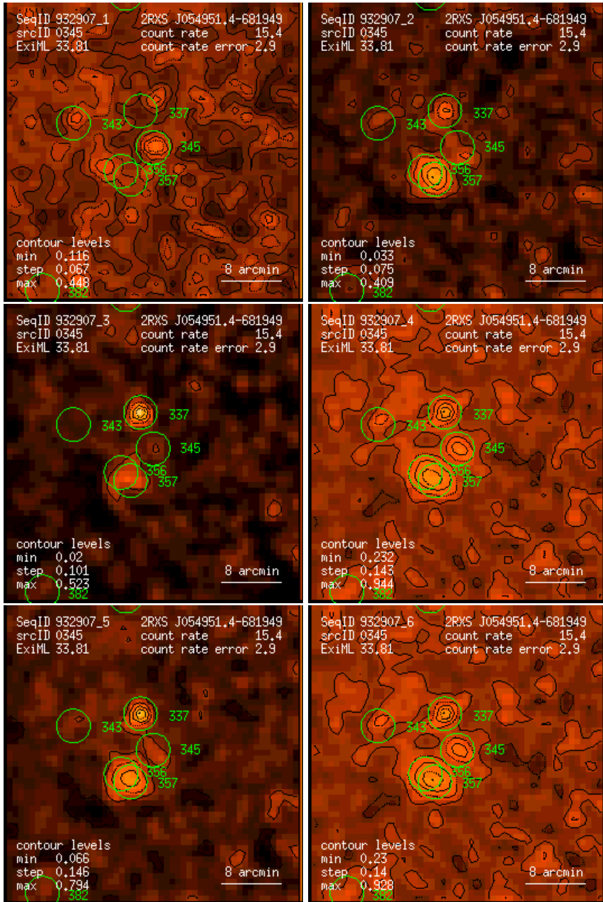
Figure 345: RASS 932907: detection 0345: band rate images, Gaussian filter: (1) PSPC channels 11 – 41, (2) 52 – 90, (3) 91 – 201, (4) 11 – 235, (5) 52 – 201, (6) 11 – 201. Broad band rates in counts/ks. Band rate contour levels in counts/ks/arcmin 2 .
