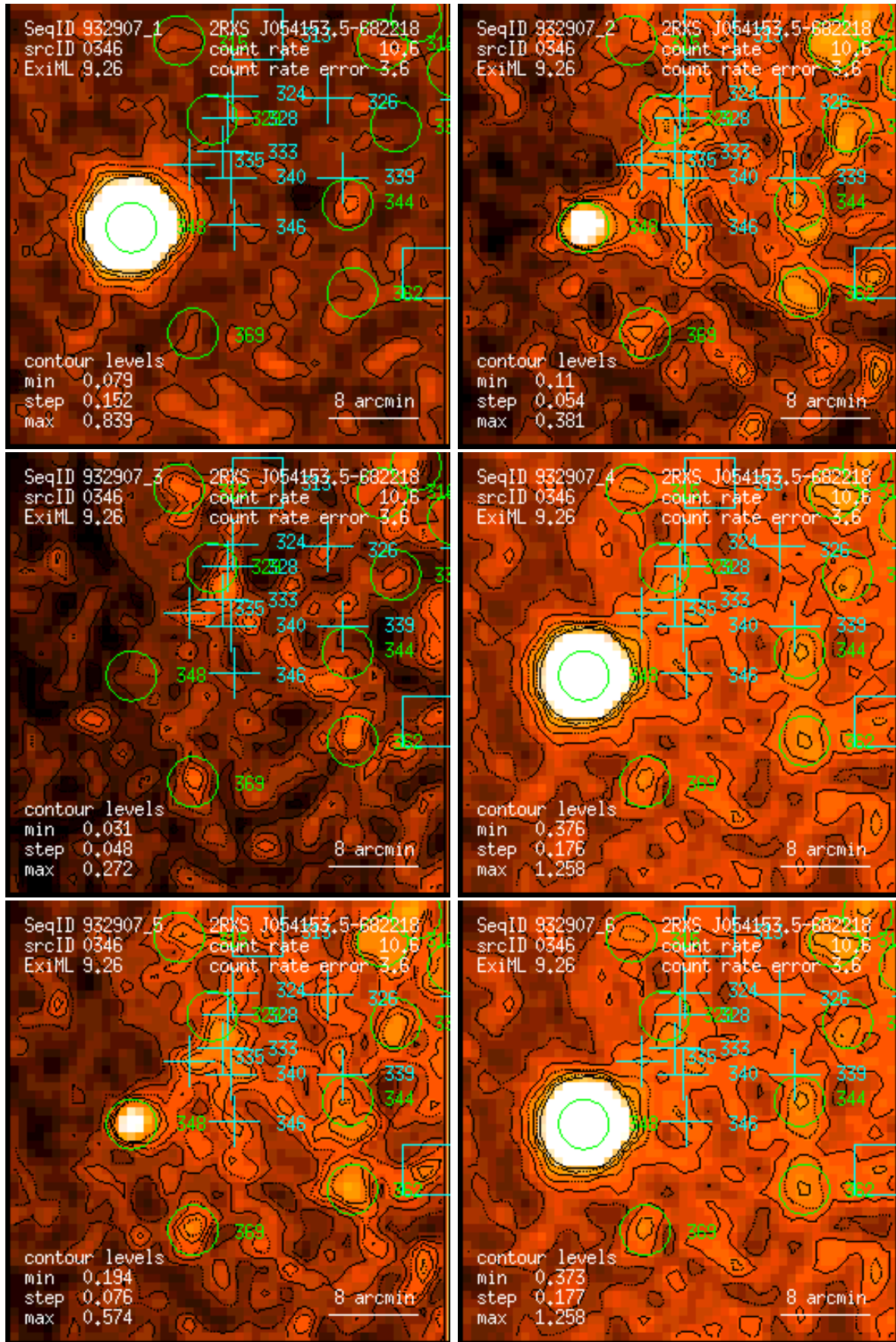
Figure 346: RASS 932907: detection 0346: band rate images, Gaussian filter: (1) PSPC channels 11 – 41, (2) 52 – 90, (3) 91 – 201, (4) 11 – 235, (5) 52 – 201, (6) 11 – 201. Broad band rates in counts/ks. Band rate contour levels in counts/ks/arcmin 2 .
