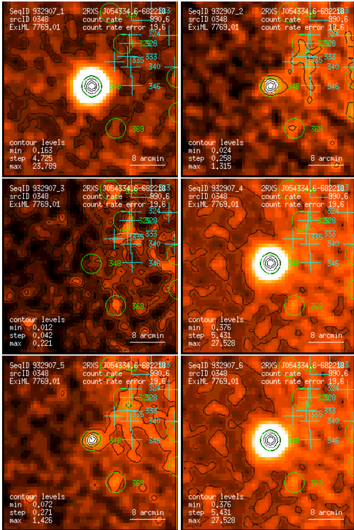
Figure 348: RASS 932907: detection 0348: band rate images, Gaussian filter: (1) PSPC channels 11 – 41, (2) 52 – 90, (3) 91 – 201, (4) 11 – 235, (5) 52 – 201, (6) 11 – 201. Broad band rates in counts/ks. Band rate contour levels in counts/ks/arcmin 2 .
