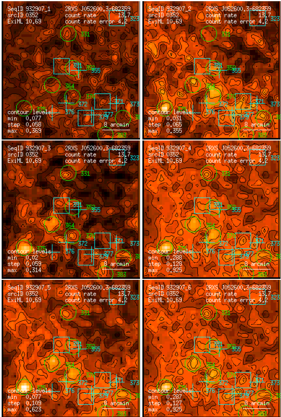
Figure 352: RASS 932907: detection 0352: band rate images, Gaussian filter: (1) PSPC channels 11 – 41, (2) 52 – 90, (3) 91 – 201, (4) 11 – 235, (5) 52 – 201, (6) 11 – 201. Broad band rates in counts/ks. Band rate contour levels in counts/ks/arcmin 2 .
