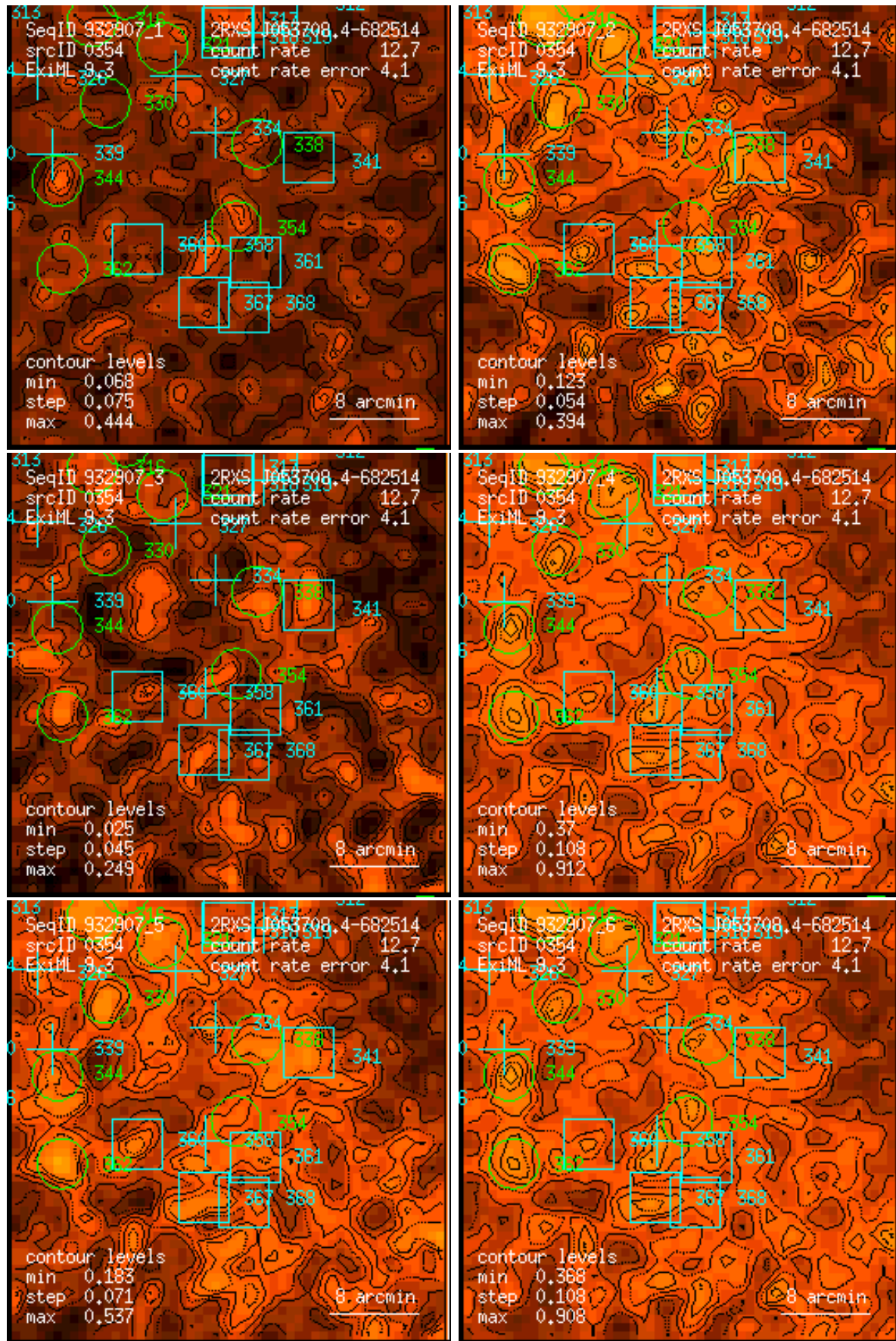
Figure 354: RASS 932907: detection 0354: band rate images, Gaussian filter: (1) PSPC channels 11 – 41, (2) 52 – 90, (3) 91 – 201, (4) 11 – 235, (5) 52 – 201, (6) 11 – 201. Broad band rates in counts/ks. Band rate contour levels in counts/ks/arcmin 2 .
