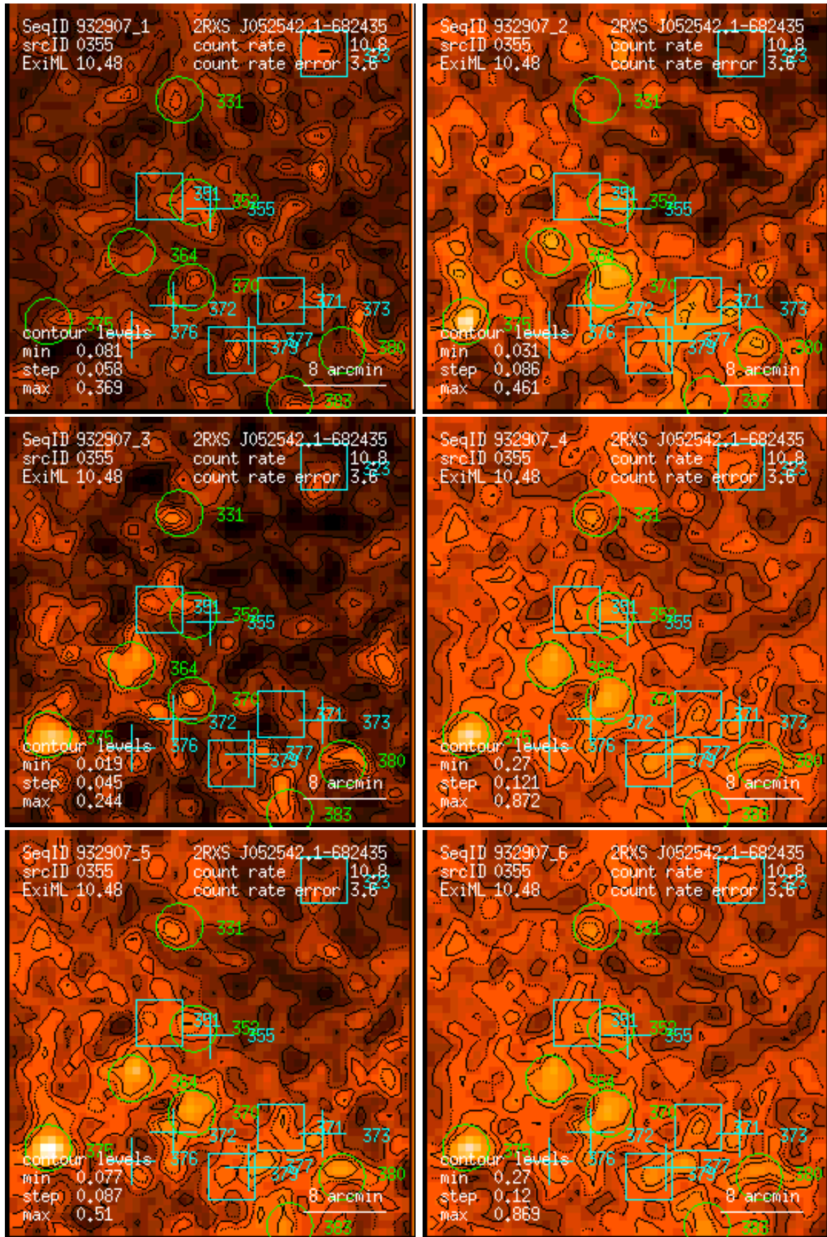
Figure 355: RASS 932907: detection 0355: band rate images, Gaussian filter: (1) PSPC channels 11 – 41, (2) 52 – 90, (3) 91 – 201, (4) 11 – 235, (5) 52 – 201, (6) 11 – 201. Broad band rates in counts/ks. Band rate contour levels in counts/ks/arcmin 2 .
