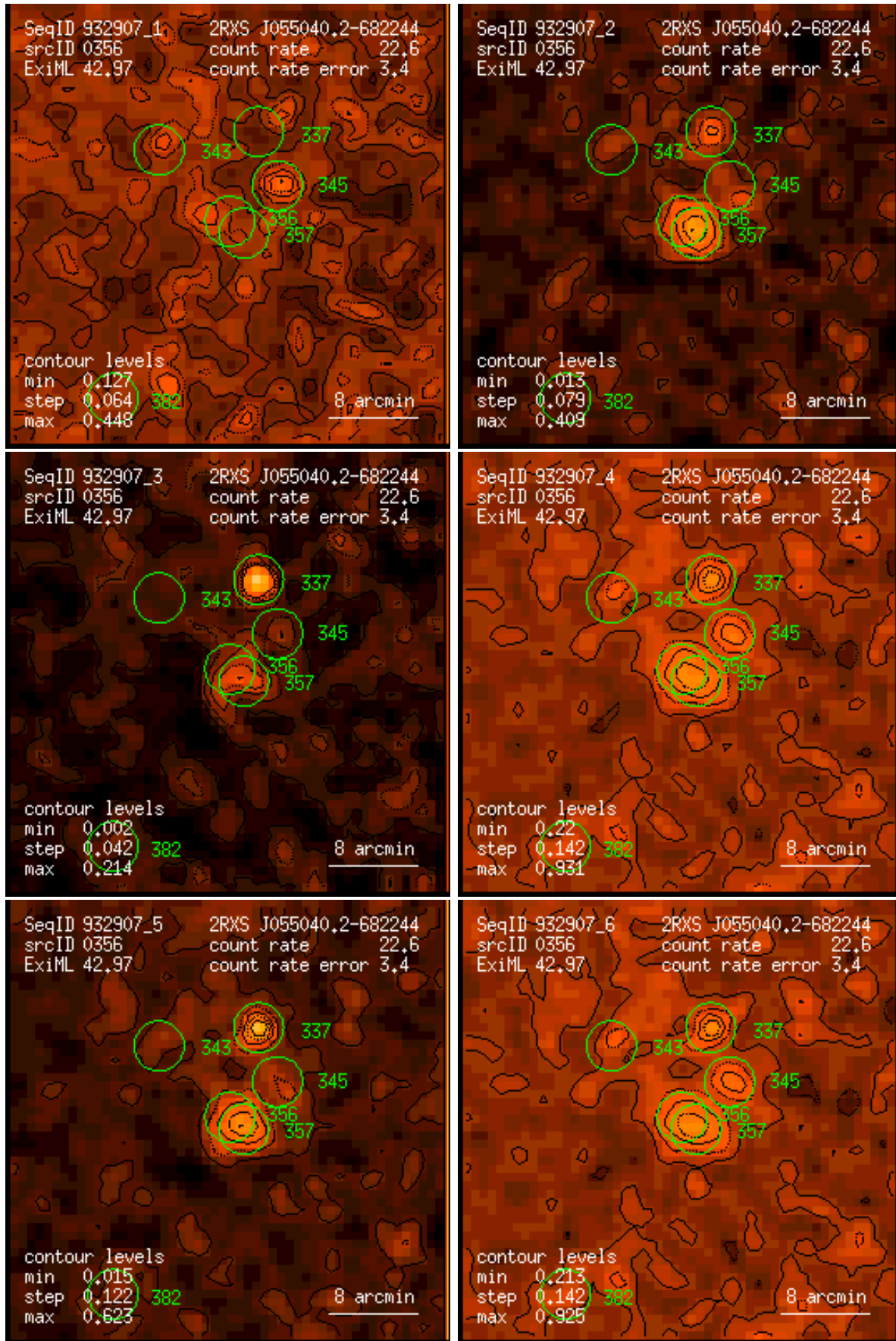
Figure 356: RASS 932907: detection 0356: band rate images, Gaussian filter: (1) PSPC channels 11 – 41, (2) 52 – 90, (3) 91 – 201, (4) 11 – 235, (5) 52 – 201, (6) 11 – 201. Broad band rates in counts/ks. Band rate contour levels in counts/ks/arcmin 2 .
