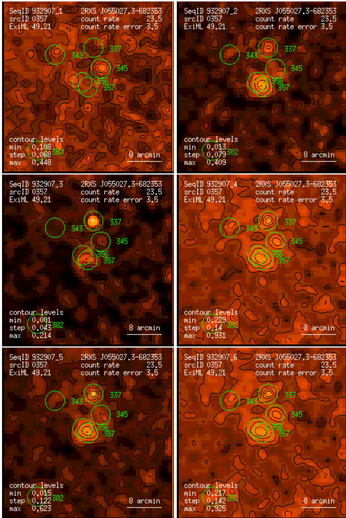
Figure 357: RASS 932907: detection 0357: band rate images, Gaussian filter: (1) PSPC channels 11 – 41, (2) 52 – 90, (3) 91 – 201, (4) 11 – 235, (5) 52 – 201, (6) 11 – 201. Broad band rates in counts/ks. Band rate contour levels in counts/ks/arcmin 2 .
