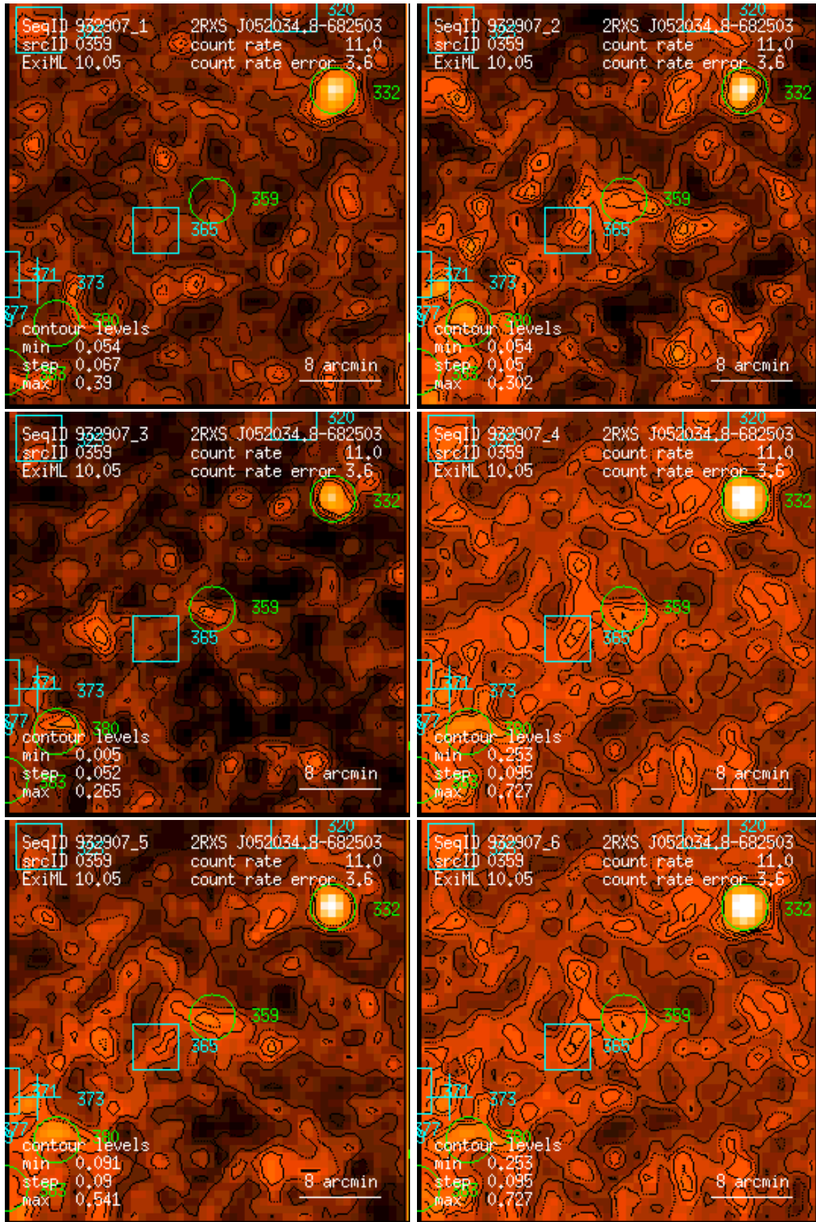
Figure 359: RASS 932907: detection 0359: band rate images, Gaussian filter: (1) PSPC channels 11 – 41, (2) 52 – 90, (3) 91 – 201, (4) 11 – 235, (5) 52 – 201, (6) 11 – 201. Broad band rates in counts/ks. Band rate contour levels in counts/ks/arcmin 2 .
