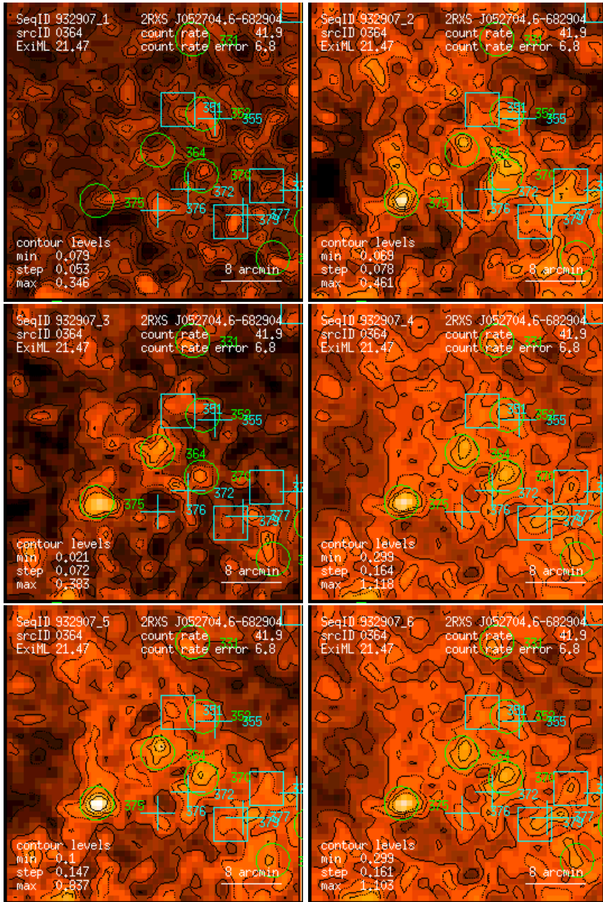
Figure 364: RASS 932907: detection 0364: band rate images, Gaussian filter: (1) PSPC channels 11 – 41, (2) 52 – 90, (3) 91 – 201, (4) 11 – 235, (5) 52 – 201, (6) 11 – 201. Broad band rates in counts/ks. Band rate contour levels in counts/ks/arcmin 2 .
