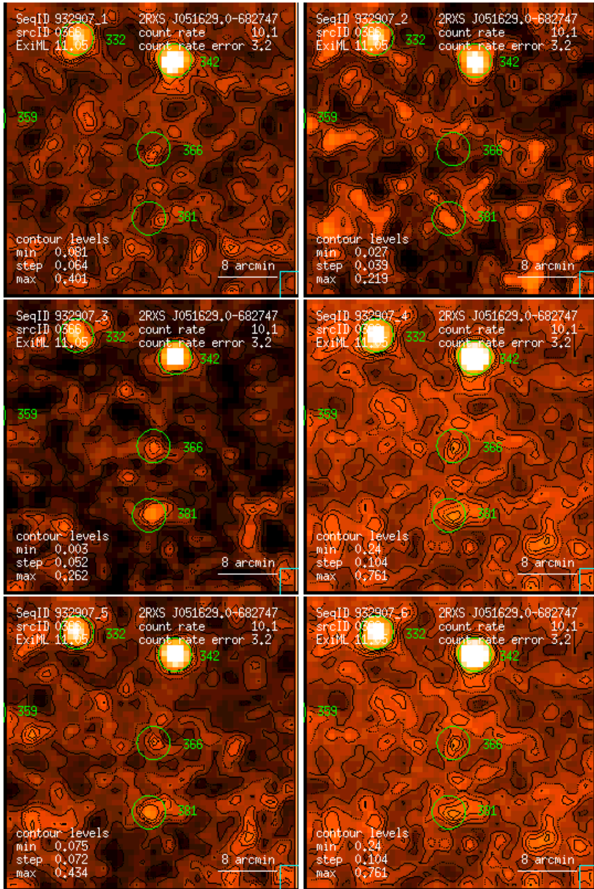
Figure 366: RASS 932907: detection 0366: band rate images, Gaussian filter: (1) PSPC channels 11 – 41, (2) 52 – 90, (3) 91 – 201, (4) 11 – 235, (5) 52 – 201, (6) 11 – 201. Broad band rates in counts/ks. Band rate contour levels in counts/ks/arcmin 2 .
